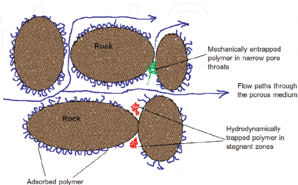
Figure 2. Retention of polymers in porous media. Sourced from [19].
