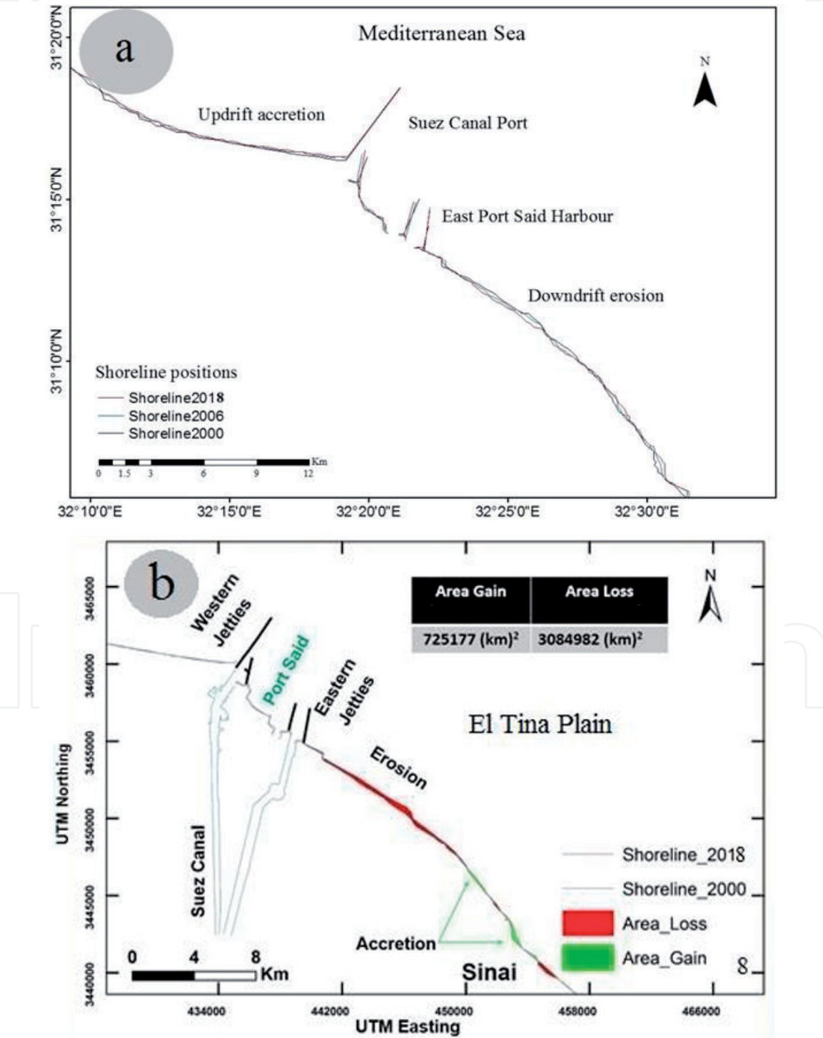
Figure 2. (a) Patterns of shoreline changes during 2000–2018 and (b) areas of loss and gain along El-Tina plain.
