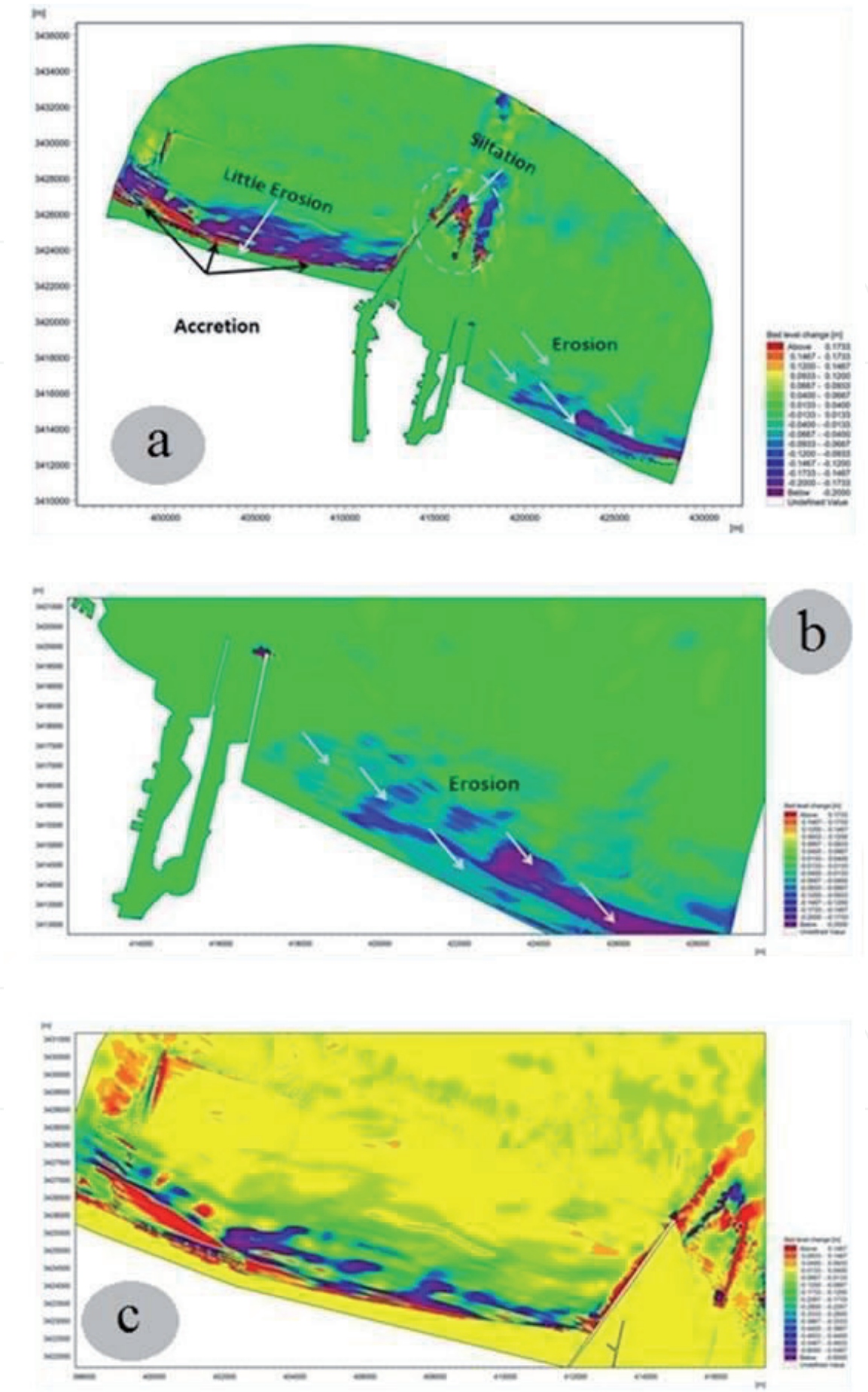
Figure 5. Modeling simulation of 10 years sediment transport during 2008–2018 along the Suez Canal coastal zone; (a) accretion along the updrift site and the entrance otherwise, erosion along the downdrift site; (b) erosion behind the eastern Jetty; and (c) siltation behind the western jetty.
