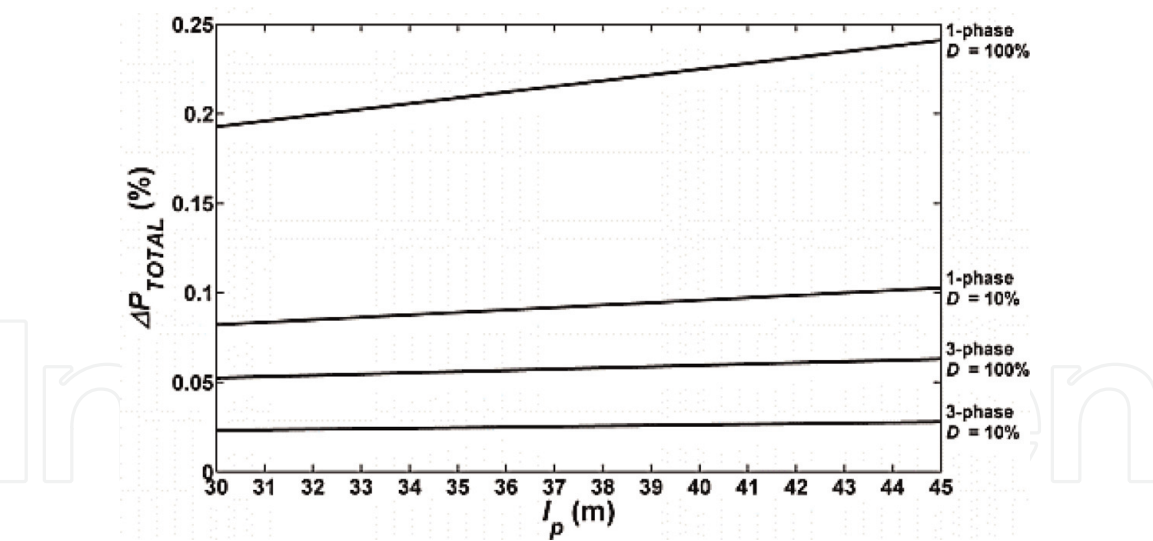
Figure 12. Relative total power losses in relation to the distance between poles for circuit consisting of three luminaires [5].
