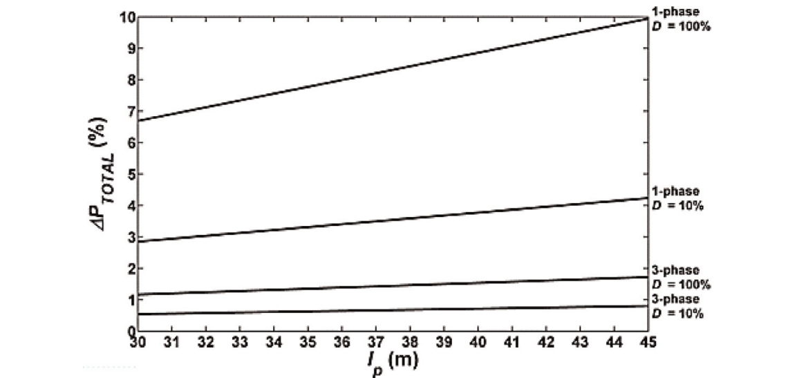
Figure 13. Relative total power losses in relation to the distance between poles for circuit consisting of 30 luminaires [5].
