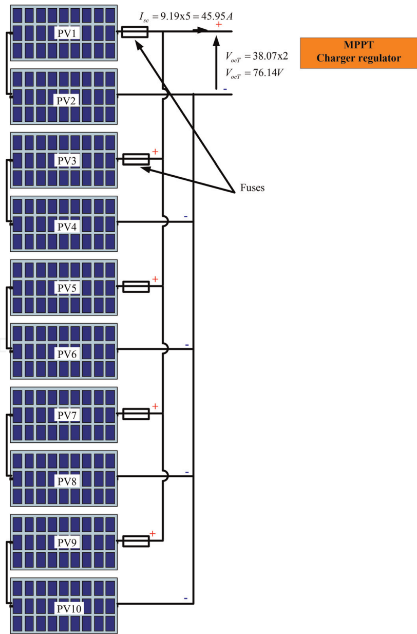
Figure 11. Fuses location in the PV system.
