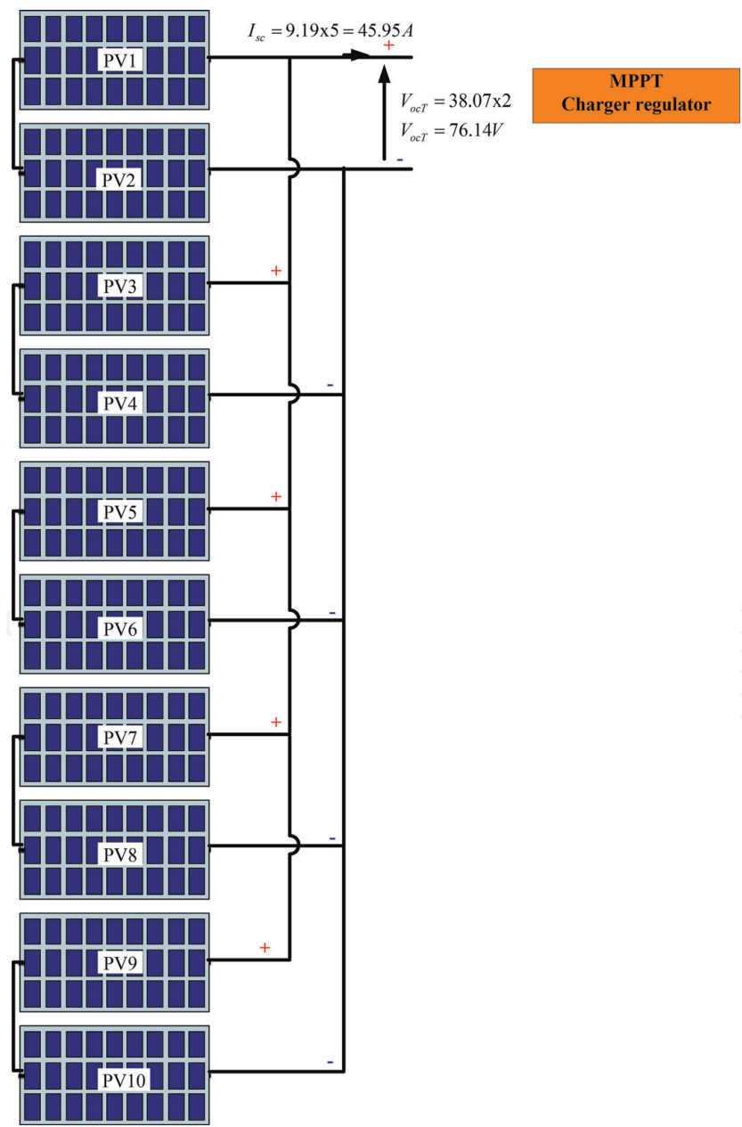
Figure 5. Photovoltaic modules association.
