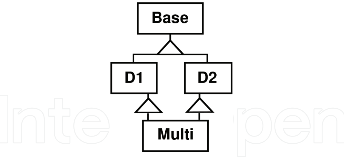
Figure 6. Diamond inheritance class diagram.
