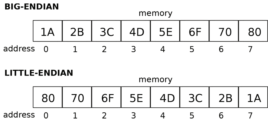
Figure 1. Representation of 0x1A2B3C4D5E6F7080 in big-endian and little-endian.
