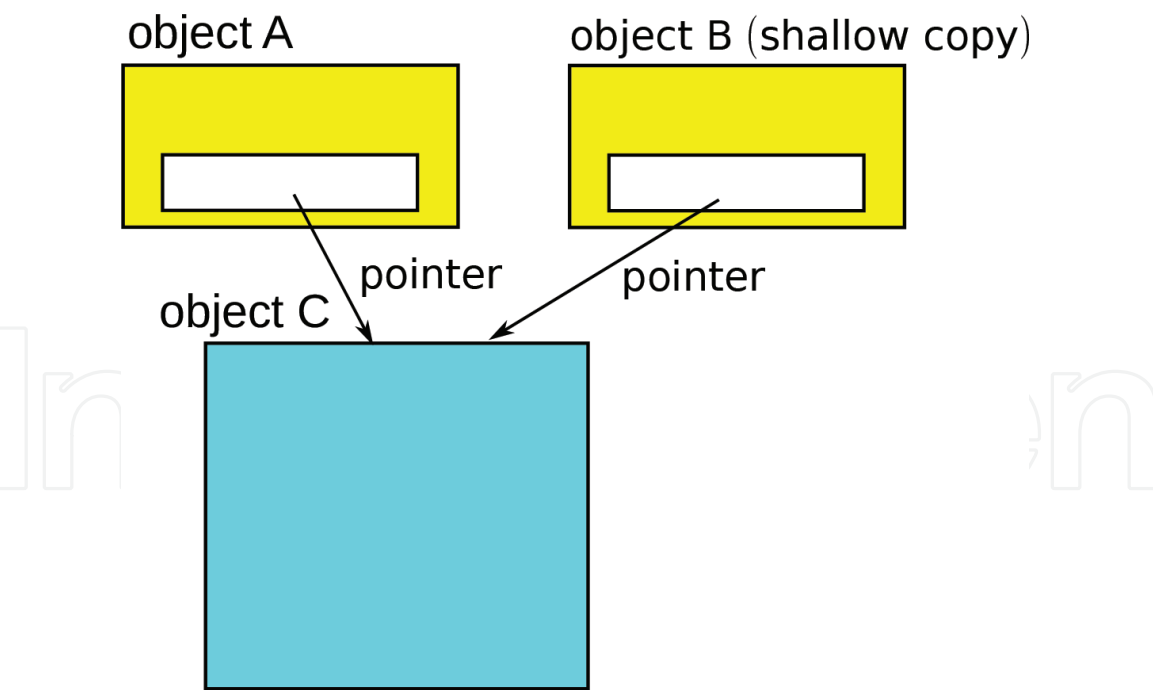
Figure 3. An example of a shallow copy.
