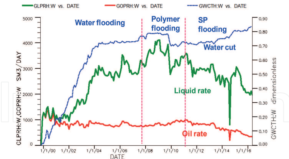
Figure 8. Field production curves in JW field.
