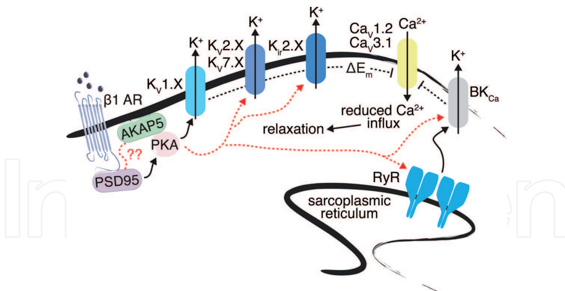
Figure 2. Regulation of vascular smooth muscle excitability by K^+ channels. Vascular smooth muscle cells express a number of K^+ channels that, upon activation, provide negative feedback regulation of membrane potential and vascular tone. K^+ channel activation results in efflux of K^+ ions that hyperpolarize the membrane potential ( \Delta E_m ; denoted by dotted black lines) leading to a reduction in the open probability of LTCC Ca_v1.2 and TTCC Ca_v3.1 that results in a decrease in global [Ca^{2+}]_i leading to vascular smooth muscle relaxation [32, 95]. As mentioned in Figure 1 , activation of ryanodine receptors (RyR) K^+ channels can be distinctively regulated by vasoactive agents acting through the G_s/AC/PAK , NO/sGC/PKG , and G_q/PLC/PKC axes to either increase or decrease their activity. An example is the regulation of K_{V1.X} channels by \beta adrenergic signaling (e.g., through \beta_1 adrenergic receptors) [44–46]. Here, K_{V1.X} channel regulation by \beta_1 adrenergic signaling requires PKA targeting to the channel by postsynaptic density protein 95 (PSD95). Whether PSD95 as well as further scaffolding of proteins by AKAP5 is required for PKA regulation of K_{V1.X} and other K^+ channels (e.g., K_{V2.X} , K_{V7.X} , K_{ir2.X} ) as well as RyR is unclear (denoted by dotted red lines in the cartoon). The model was generated by taking in consideration studies cited and described above. K^+ = potassium; Ca^{2+} = calcium; AKAP5 = A kinase anchoring protein 5; BK_{Ca} = large-conductance Ca^{2+} activated potassium channels; AC = adenylyl cyclase; PKA = protein kinase A; NO = nitric oxide; sGC = soluble guanylyl cyclase; PKG = protein kinase G; PLC = phospholipase C; PKC = protein kinase C.
