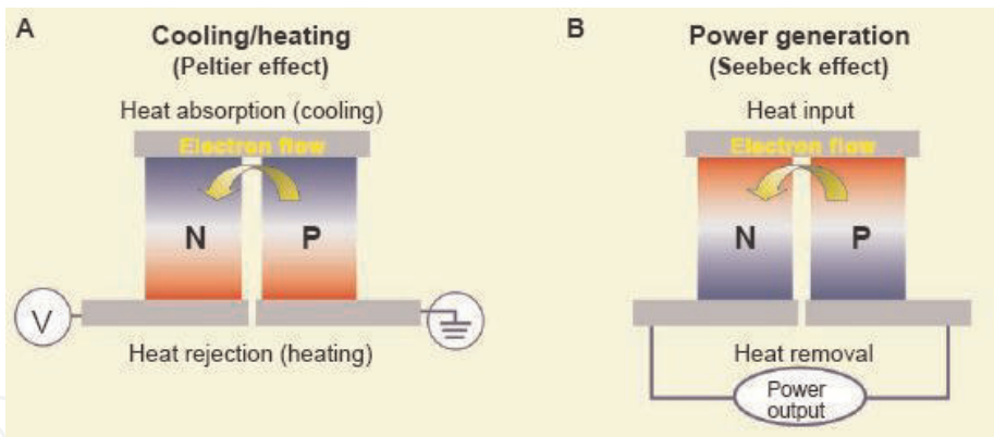
Figure 1. Thermoelectric principle.
