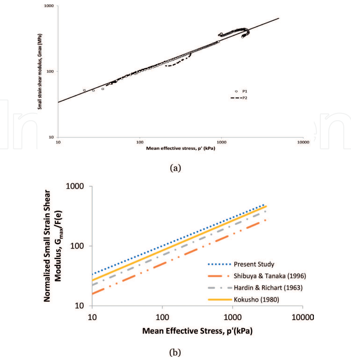
Figure 10. Variation of G_{max} with p' for uncemented sand (a) dry and saturated Sydney sand (b) validation with published data.
