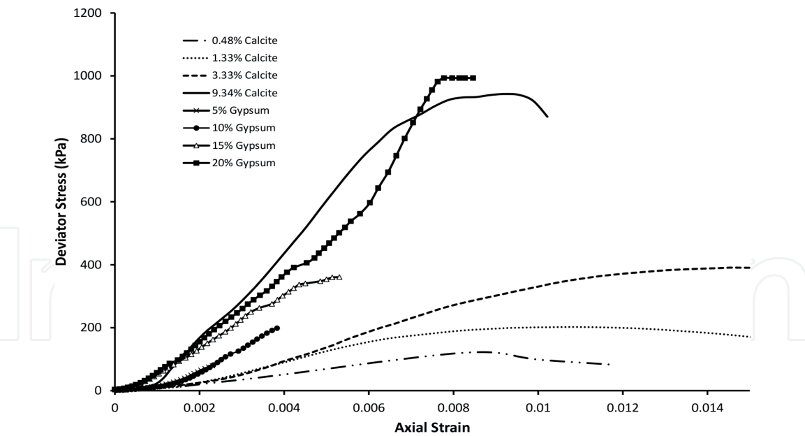
Figure 3. Comparison of UCS responses of gypsum and bio-cemented specimens.
