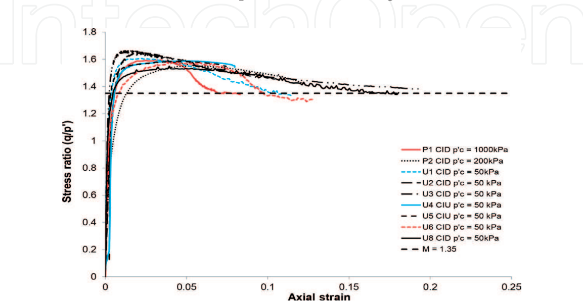
Figure 8. Response of uncemented Sydney sand.
