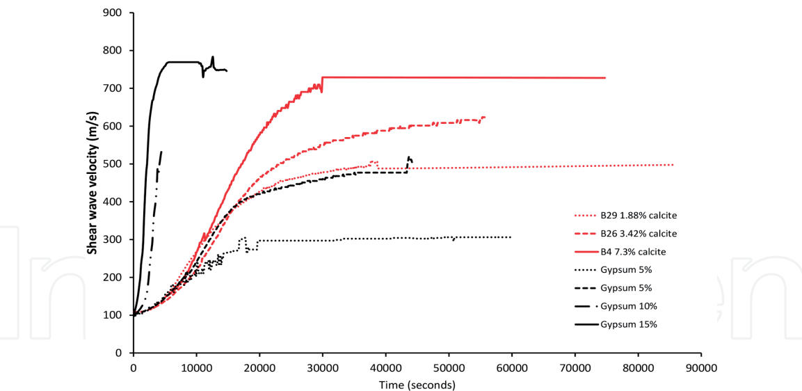
Figure 7. Comparison of curing for gypsum and bio-cemented specimens.
