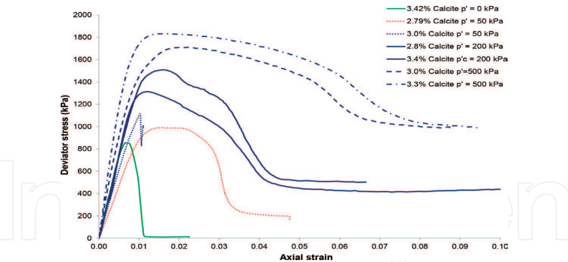
Figure 19. Deviator stress, axial strain responses for bio-cemented specimens (2.8–3.4% calcite).
