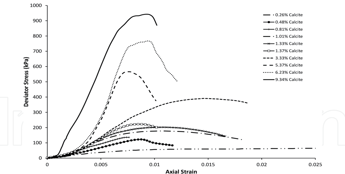
Figure 2. UCS responses for bio-cemented specimens.
