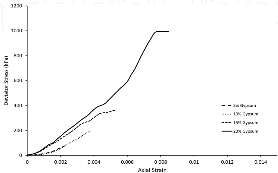
Figure 1. UCS test responses from gypsum-cemented specimens.
