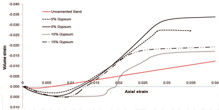
Figure 13. Volume strain, axial strain responses from drained tests ( p'_c = 50 \text{ kPa} ).
