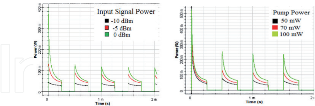
Figure 17. EDFA transient response to signal (left) and pump variations (right).
