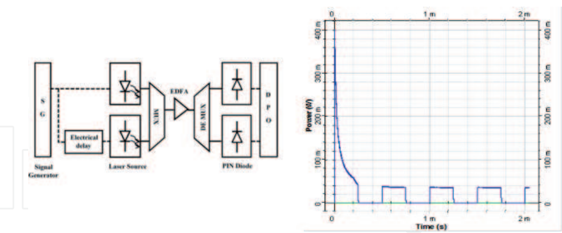
Figure 20. Compensation using electrical delayed pulse. Schematic (left) and result (right).
