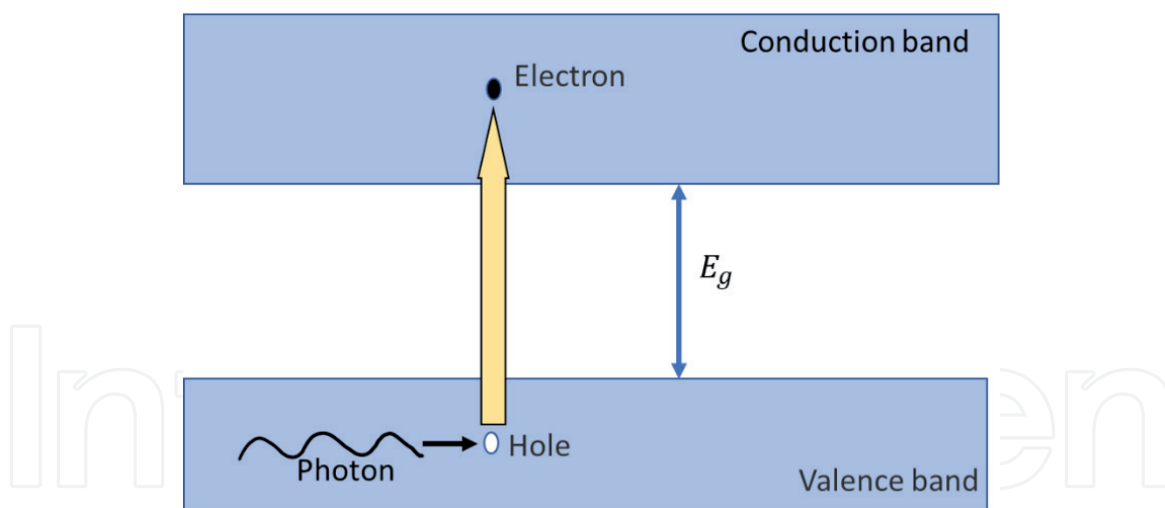
Figure 11. Photodiode basic principle.
