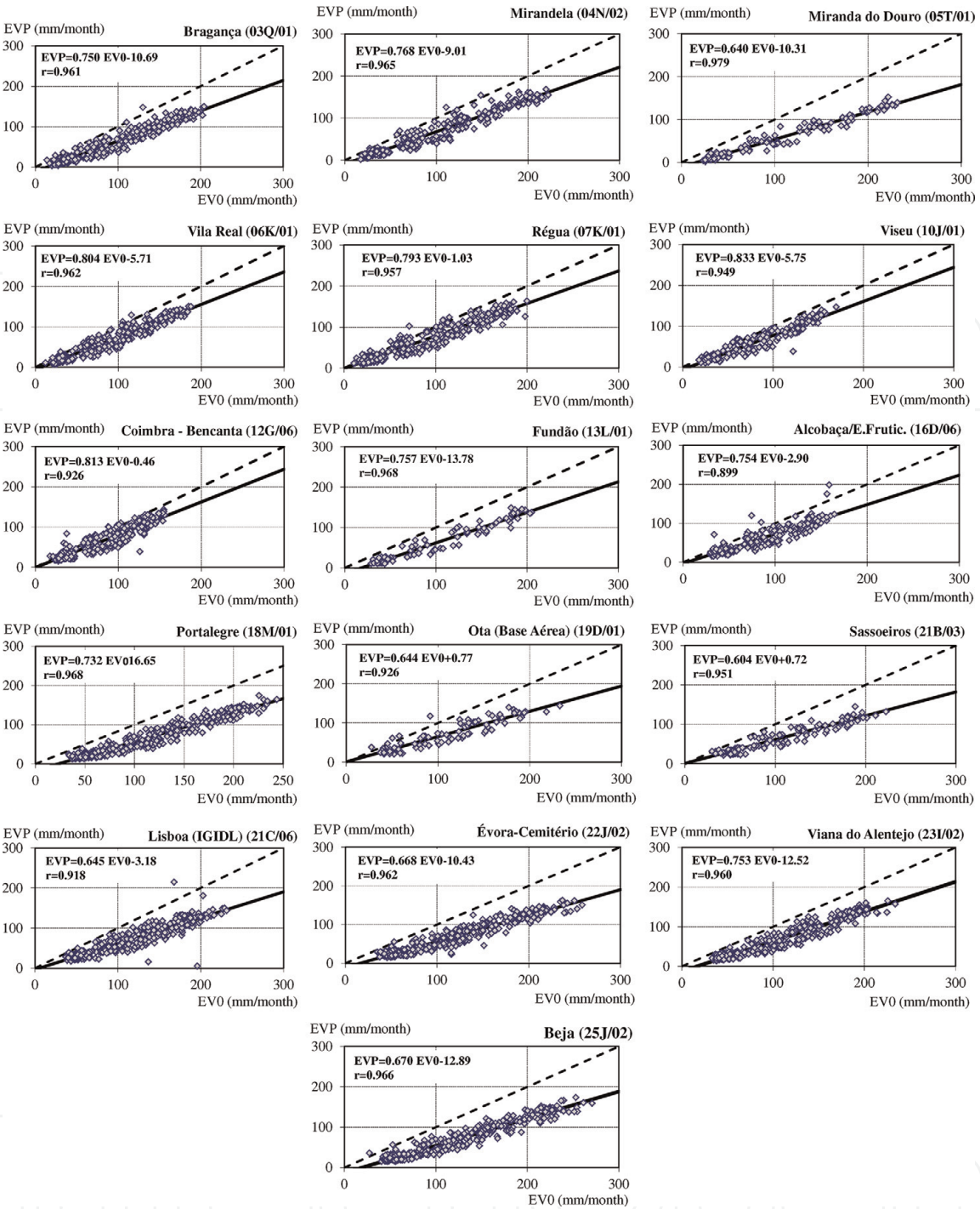
Figure 3. Monthly potential evapotranspiration of Thornthwaite, EVP, and of Penman-Monteith, EV0. Linear regression line (continuous line), equation, and correlation coefficient, r . Line representing the equality between monthly EVP and EV0 (dashed line).
