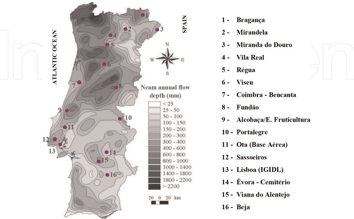
Figure 1. Location of the climatological stations of Table 1.
