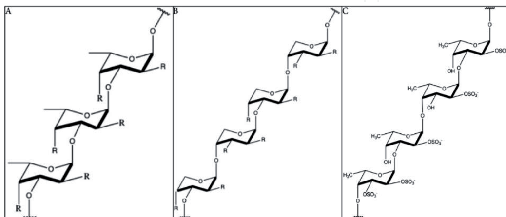
Figure 6. Structure of fucoidans [54].
