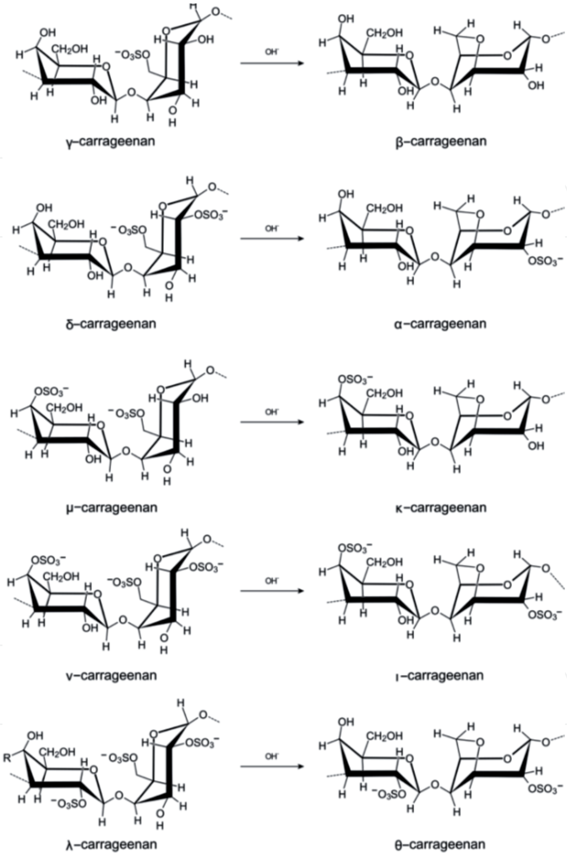
Figure 7. Chemical structure of carrageenans [57].
