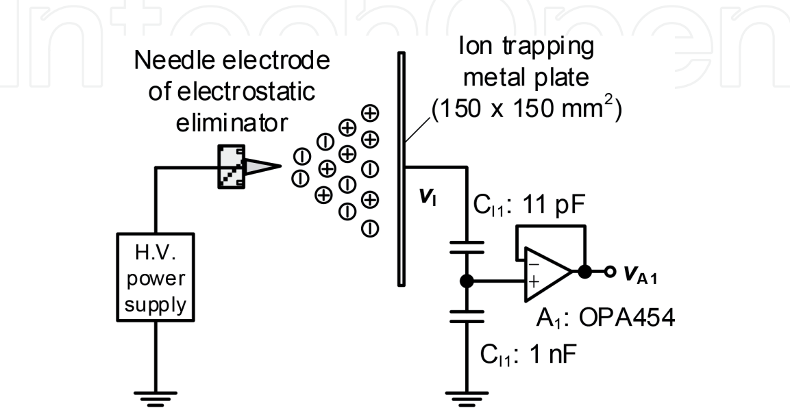
Figure 8. Schematic diagram of the ion measuring system.
