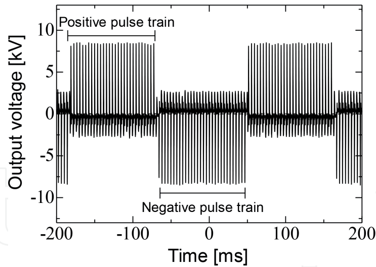
Figure 6. Typical waveform of continuously generated pulse train [26].
