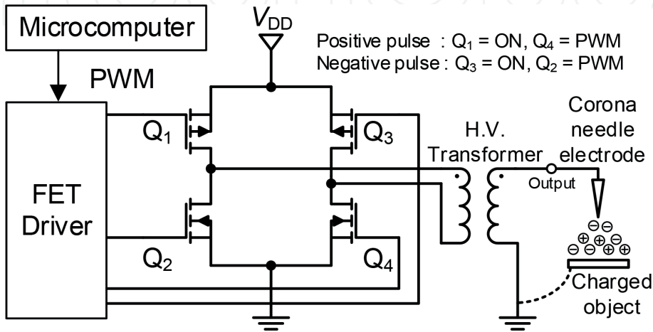
Figure 3. Schematic diagram of the bipolar pulse voltage power supply driven by a full-bridge PWM converter [26].
