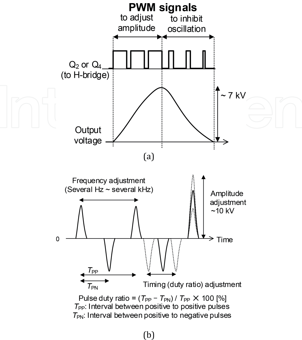
Figure 4. Schematic diagram of PWM control [26]. (a) Relationship between the output voltage and the control signals, (b) output voltage.
