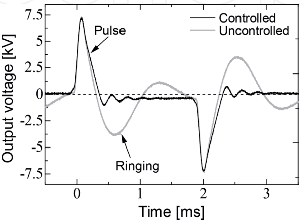
Figure 5. Typical waveform of output voltage [26].
