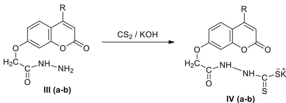
Figure 6. Synthesis of coumarin potassium salts IV(a-b) .
