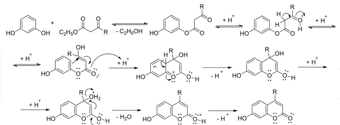
Figure 3. Mechanism of the Pechmann condensation.
