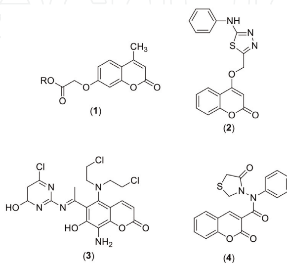
Figure 1. Coumarin derivatives with antimicrobial activity.
