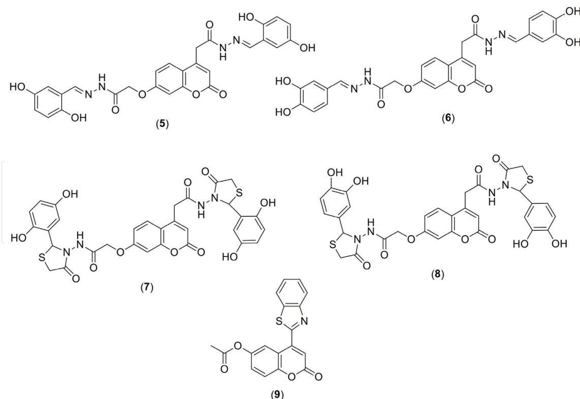
Figure 2. Coumarin derivatives with antioxidant activity.
