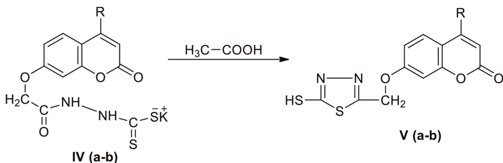
Figure 7. Synthesis of coumarin thiadiazoles derivatives V(a-b) .
