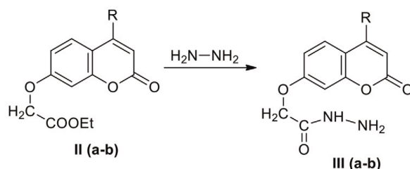
Figure 5. Synthesis of coumarin acetohydrazides III(a-b) .
