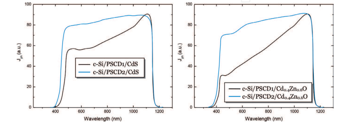
Figure 15. Spectral distribution of photocurrent for heterojunctions c-Si/PSCD/CdS and c-Si/PSCD/Cd 0.4 Zn 0.6 O based on PSCD1 and PDCS2 substrates [19–22].
