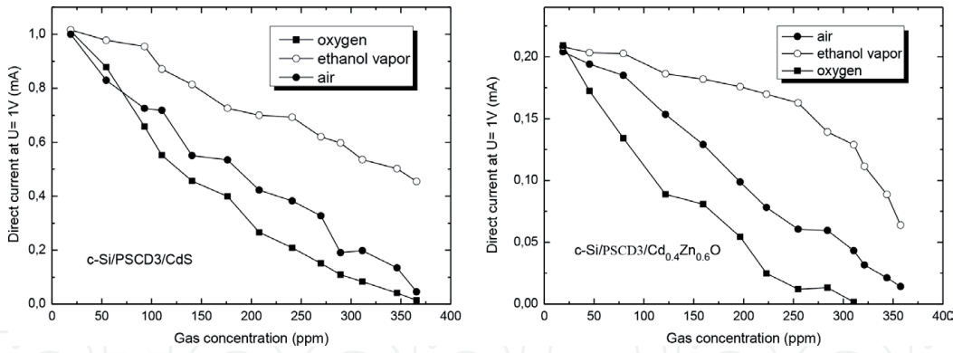
Figure 12. Dependence of direct current at U = 1 V on the concentration of different gases for heterojunctions c\text{-Si/PSCD3/CdS} and c\text{-Si/PSCD3/Cd}_{0.4}\text{Zn}_{0.6}\text{O} .
