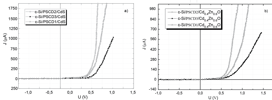
Figure 10. Dark J - V curves for as-deposited c -Si/PS/CdS and c -Si/PS/Cd 0.4 Zn 0.6 O heterojunctions prepared onto the PSCD1, PSCD2, and PSCD3 substrates.
