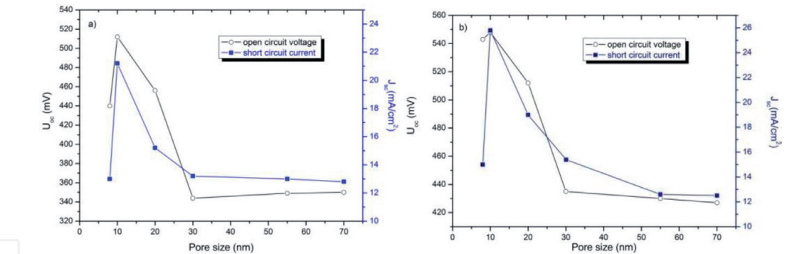
Figure 14. Dependences of U_{oc} and J_{sc} on the pore size in silicon for heterojunctions c-Si/PSCD/Cd 0.4 Zn 0.6 O (a) and c-Si/PSCD/CdS (b).
