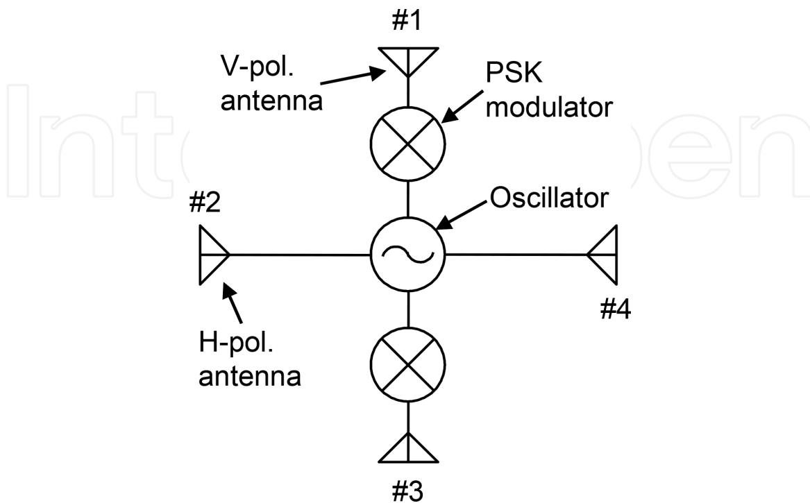
Figure 5. Basic block diagram of the active integrated array antenna [9].
