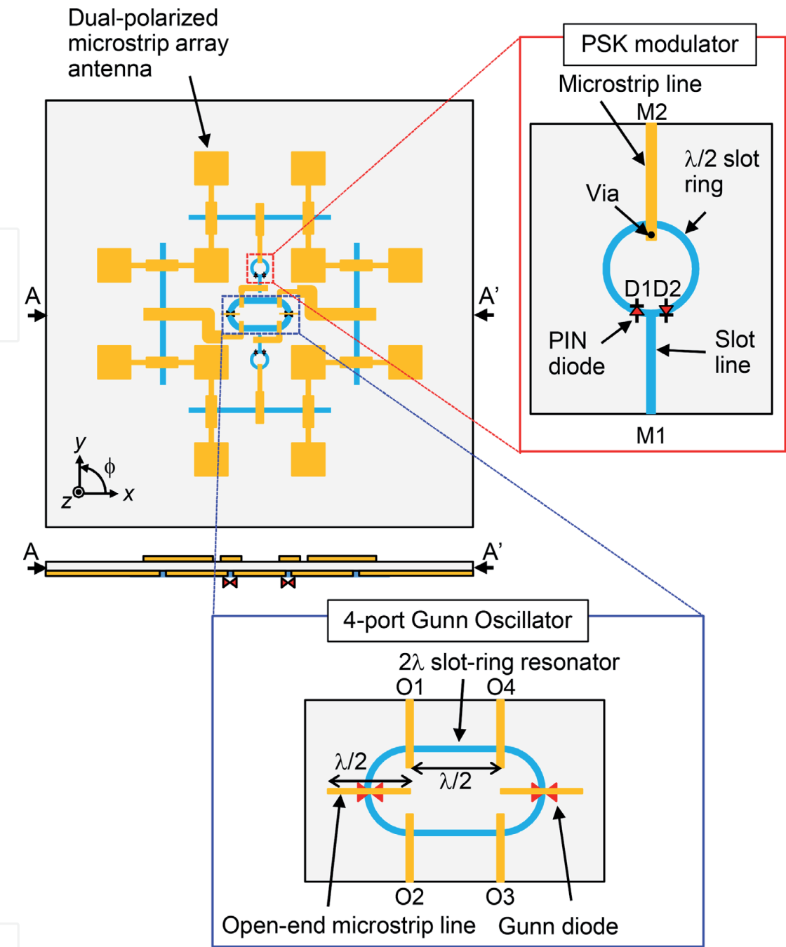
Figure 6. Structure of the active integrated array antenna [10].
