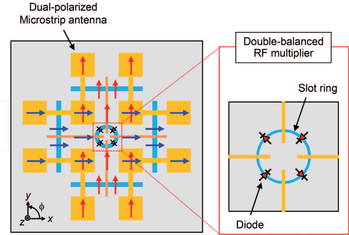
Figure 8. Polarization discrimination antenna [11].
