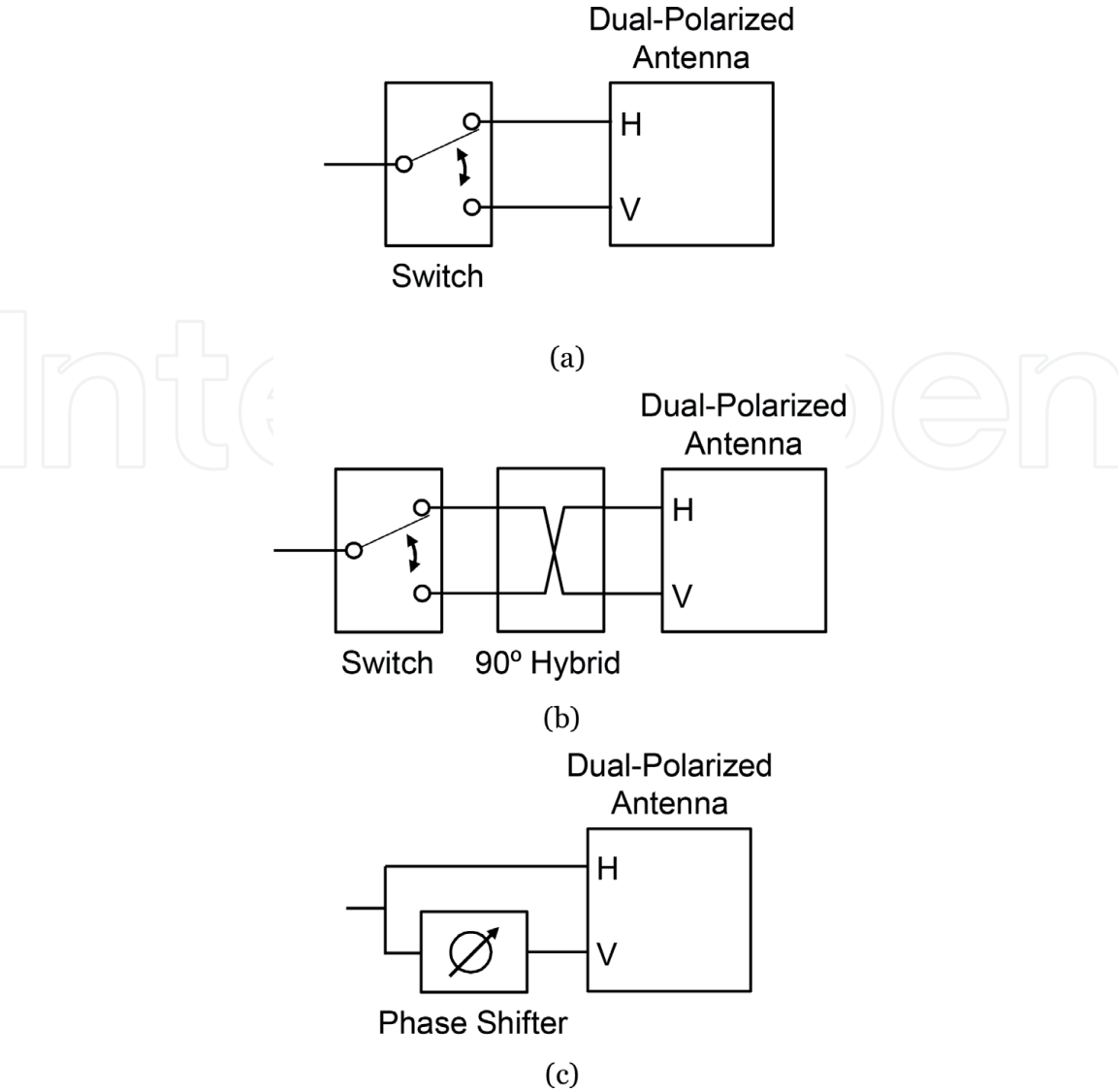
Figure 3. Basic configurations of polarization agile antenna. (a) Linear polarization switchable antenna; (b) circular polarization switchable antenna and (c) linear/circular polarization switchable antenna.
