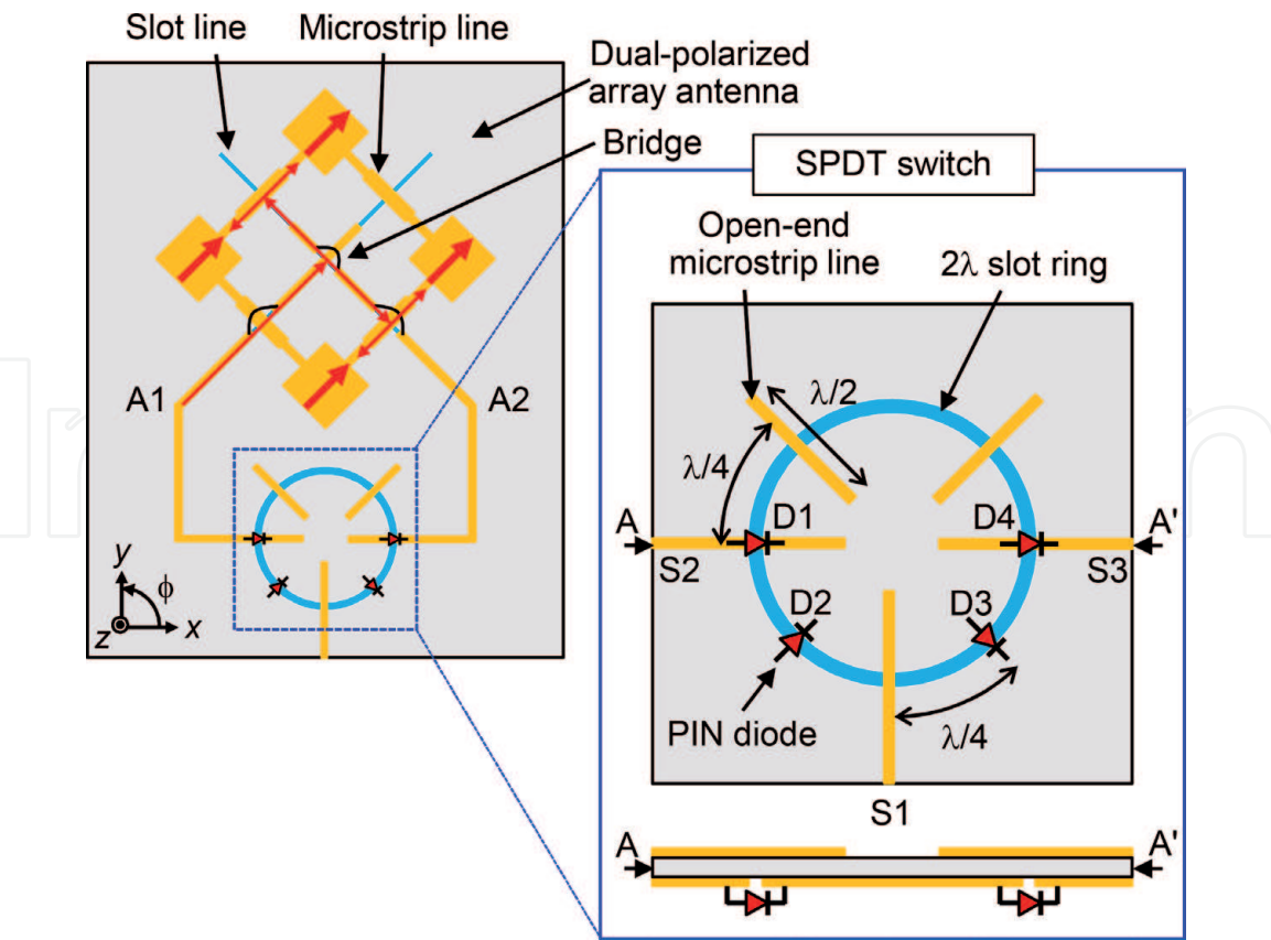
Figure 4. Structure of a linear polarization switchable antenna [3].
