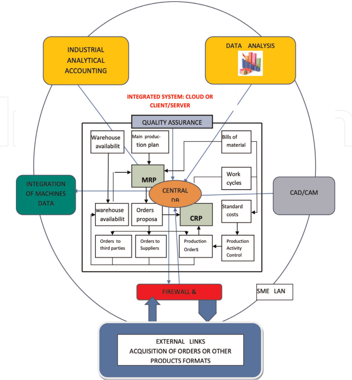
Figure 2. Scheme showing the main interconnections to the corporate network, to the CAD/CAM.
