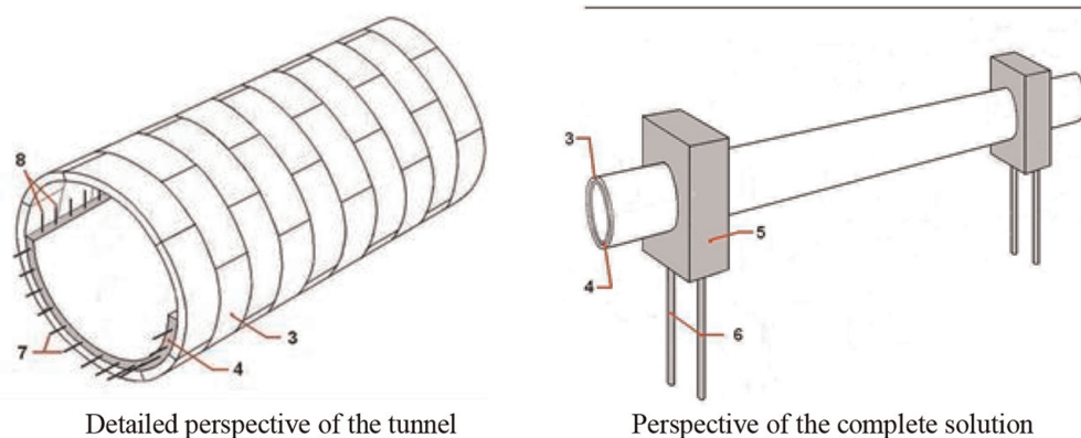
Figure 4. Illustration of the TISB concept.
