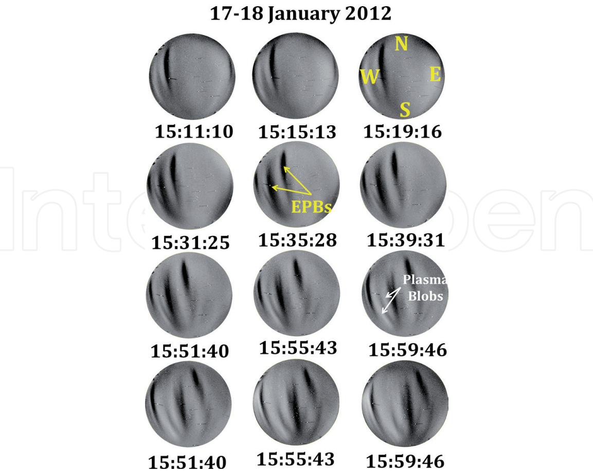
Figure 1. Sequences of images of OI 630.0 nm obtained on 17-18 January, 2012 in IST at Kolhapur. Yellow and white arrows are showing dark and bright (EPB and plasma blob) respective structures in images.
