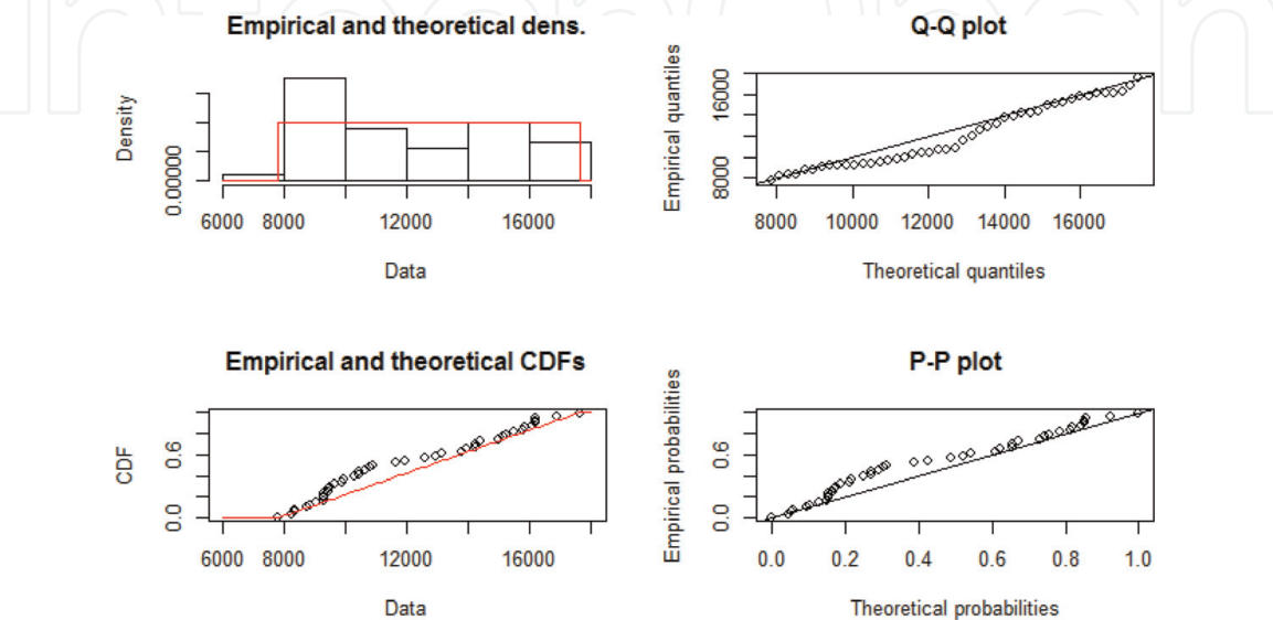
Figure 14. CO 2 emission distribution.
