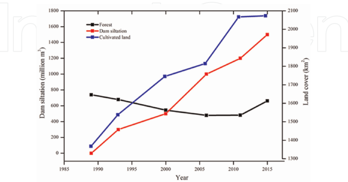
Figure 5. Changes in forest, cultivated land in the catchment area, and siltation volume in the Nkula Dam from 1989 to 2015.
