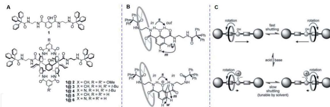
Figure 6. (A) Various [2] rotaxanes by Gschwind and coworkers [24]. (B) Interactions in a [2] rotaxane. (C) Cartoon representation illustrating the dynamic processes in the acid-/base-regulated switching of [2] rotaxanes depicted in (A). Reprinted with permission from Gschwind and coworkers [24].
