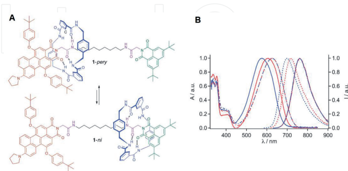
Figure 10. (A) Shuttle movement in a [2] rotaxane and (B) solvatochromic shifts observed. Reprinted with permission from Günbaş et al. [39].
