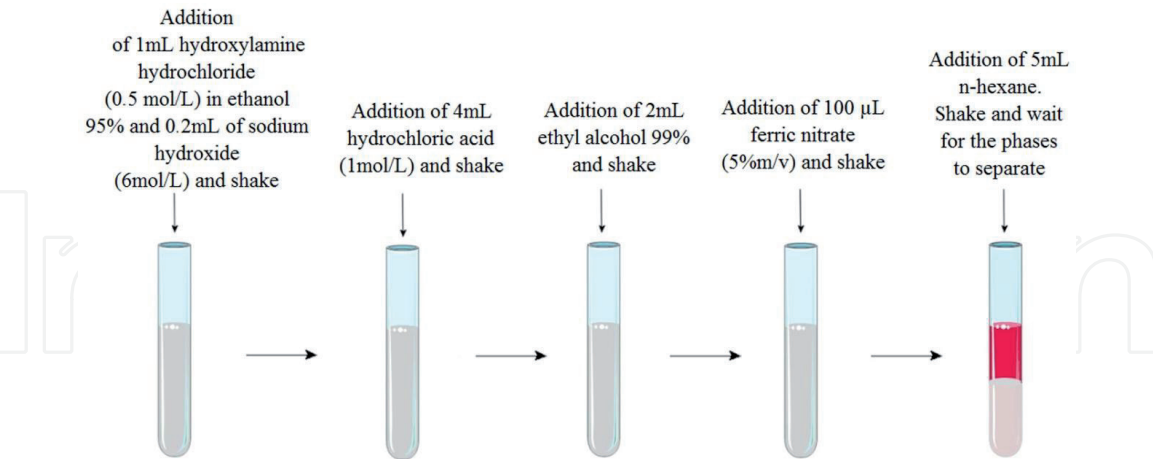
Figure 5. Schematic representation of hydroxamic acid colorimetric test. Adapted from Costa [34].
