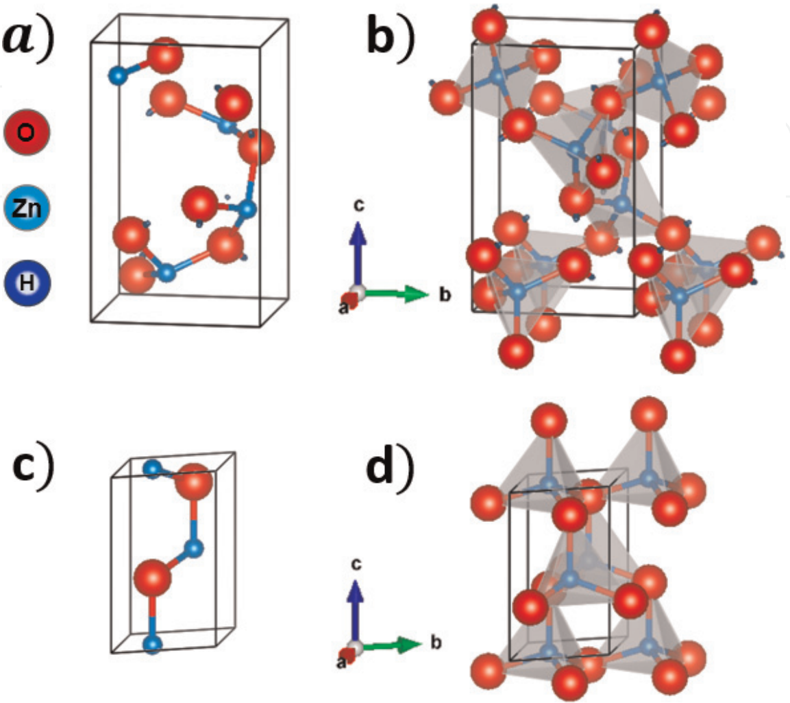
Figure 3. (a) Unitary cell of \epsilon\text{-Zn(OH)}_2 , (b) representation of polyhedra of the unitary cell of the wulfingite, (c) unitary cell of ZnO, and (d) representation of polyhedra of the unit cell of the wurtzite.
