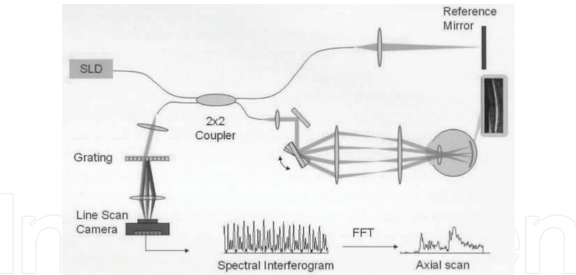
Figure 2. Principle of Fourier domain optical coherence tomography.
