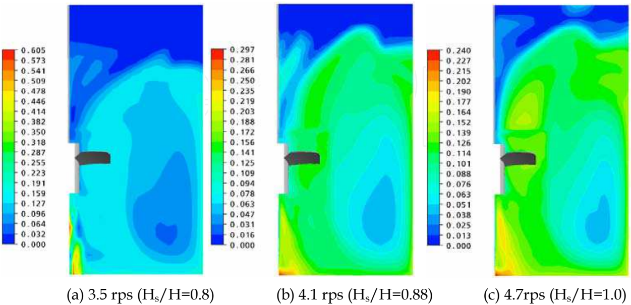
Fig. 5. Cloud height predicted by CFD simulation for A315 hydrofoil impeller at different rotational speeds (particle size of 350 \mu\text{m} with solid loading of 10 vol. %)
