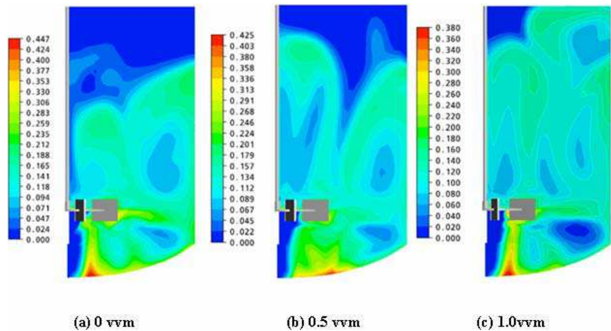
Fig. 10. Effect of air flow rate on solid concentration distribution for DT by CFD simulations at the critical impeller speed (a) 0 vvm (b) 0.5 vvm (c) 1. 0 vvm (particle size=230 \mu m and particle loading = 30 wt. %)
