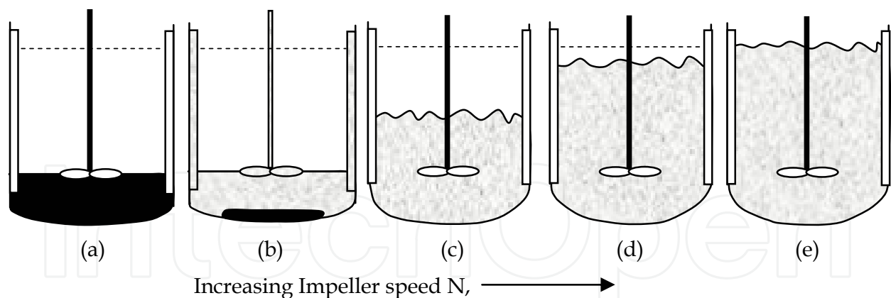
Fig. 1. Flow regimes of liquid-solid stirred reactor (Kraume, 1992)
