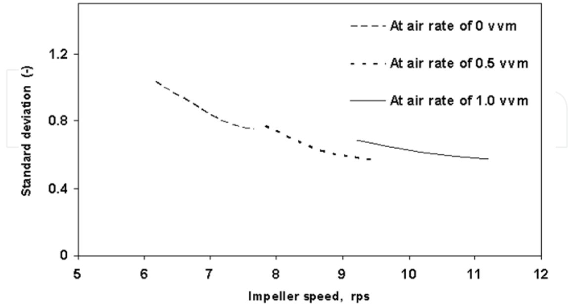
Fig. 11. Effect of gas flow rate on the standard deviation value for different impeller speeds of DT (particle size= 230 \mu m &particle loading= 30 wt.%)
