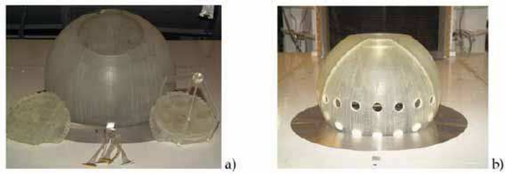
Fig. 5. VLOT wind tunnel model: (a) pressure-instrumented mirror with tubing, enclosure with tubing runs and (b) force mirror assembly (Cooper et al. , 2005)
