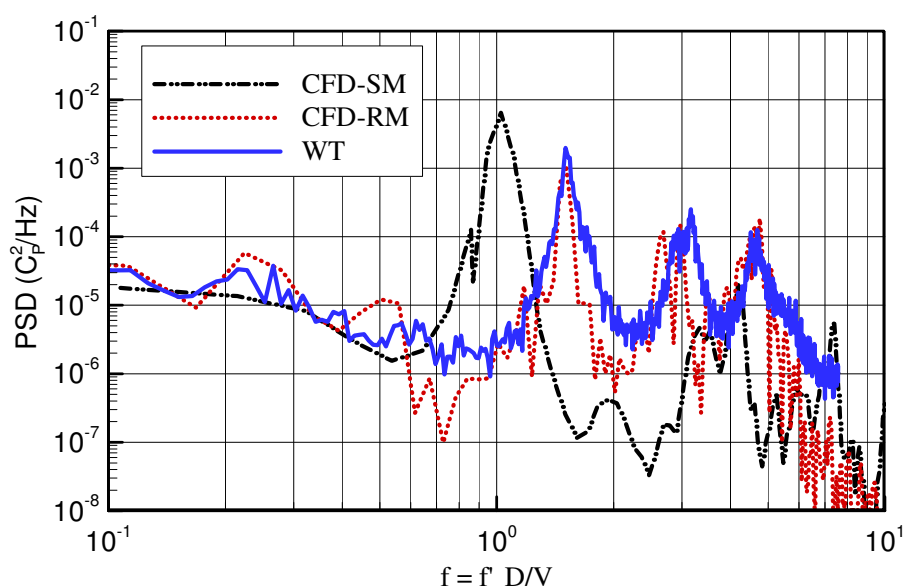
Fig. 16. CFD and experimental power density spectra pressure coefficients collected on one of the mirror probes, R4C3 ( \phi = 30^\circ and \phi = 30^\circ ) (Mamou et al. , 2008)
