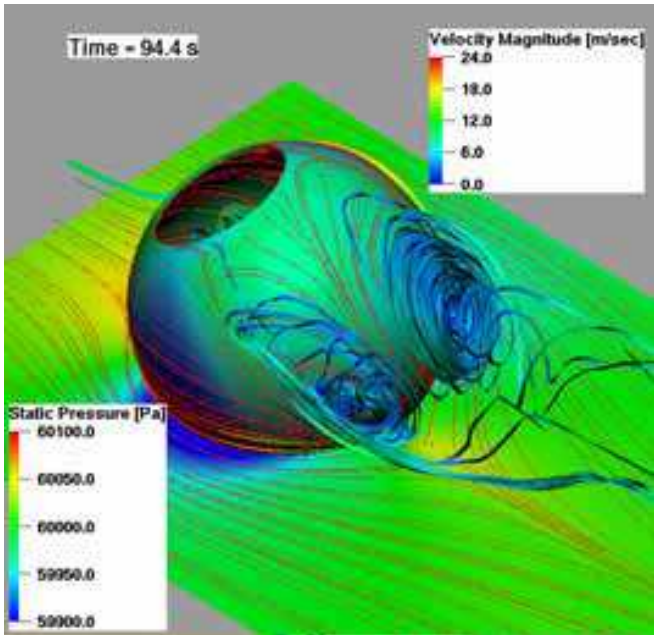
Fig. 18. Snapshot of the off-body streamlines within the separated region behind the enclosure ( \phi = 30^\circ and \varphi = 30^\circ ) (Mamou et al. , 2004a)
