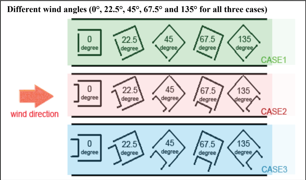
Fig. 19. Model configuration at different wind directions Figure 20 shows the physical configuration of the room model for the three cases.
