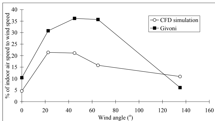
Fig. 30. Percentage of mean indoor air speed to wind speed against wind angle ranging 0° and 135° (Case 3-comparison between CFD results and the experiments of Givoni)
