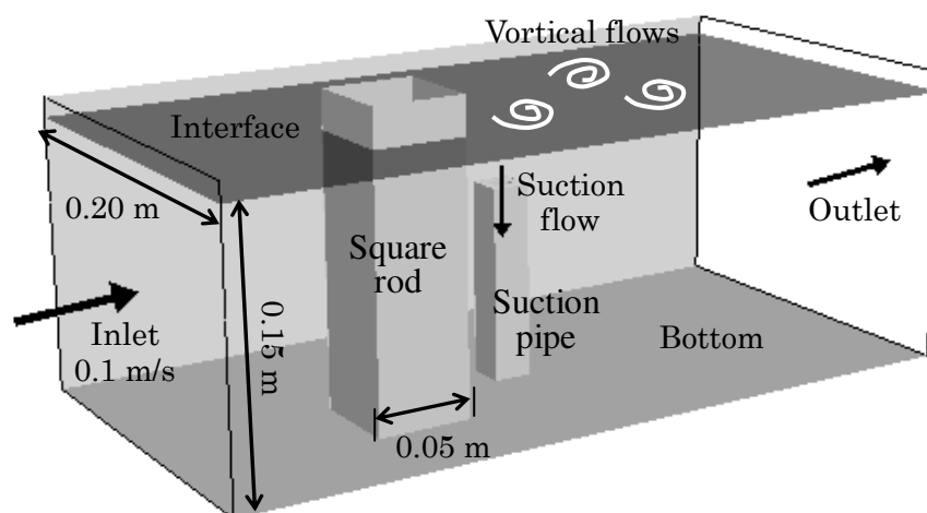
Fig. 15. Schematic view of Okamoto's experimental apparatus
