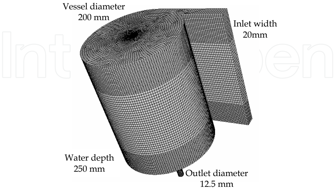
Fig. 4. Computational mesh for CFD of Monji's experiment
