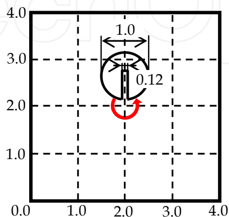
Fig. 11. Rudman's simulation conditions of slotted-disk revolution problem
