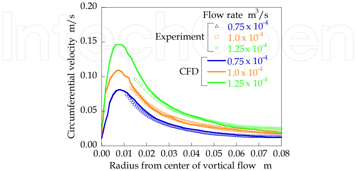
Fig. 5. Cicumferential velocity in CFD result of Moji's experiment
