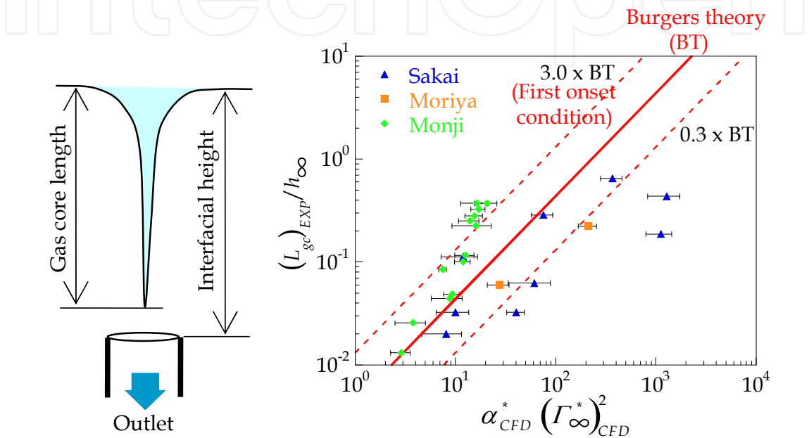
Fig. 7. Prediction accuracy of gas core length
