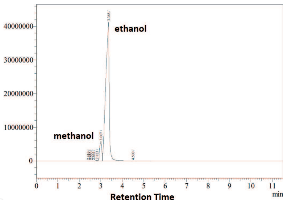
Figure 11. Example of chromatogram from the product mixture. [Reaction condition, 0.75 bar \text{CH}_4 , 2 bar \text{N}_2 contains 0.5% \text{O}_2 ; catalyst, 0.5 g Co/NaZSM-5 h; T , 150°C; t , 30 minutes].
