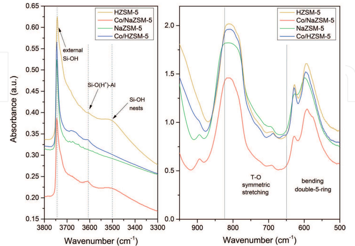
Figure 8. FTIR absorption spectra of ZSM-5 h and Co/ZSM5-h zeolites.
