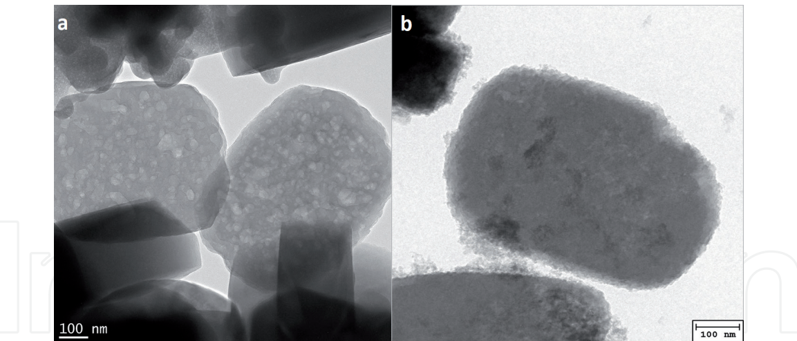
Figure 7. TEM images of (a) NaZSM-5 h and (b) Co/NaZSM5-h.
