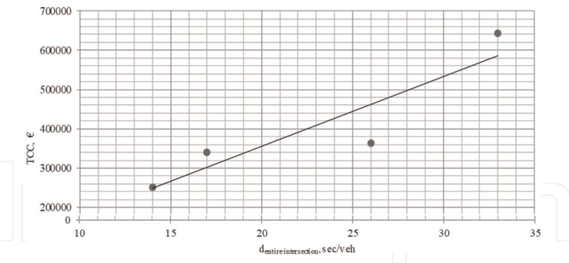
Figure 7. Total crash cost versus average control delay of the entire intersection.
