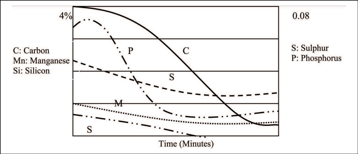
Fig. 6. Schematic representation of the progress of refining in top-blown vessel About 200 data were collected in a matrix, named with the mark of steel. A sample of the collected data is shown bellow:
