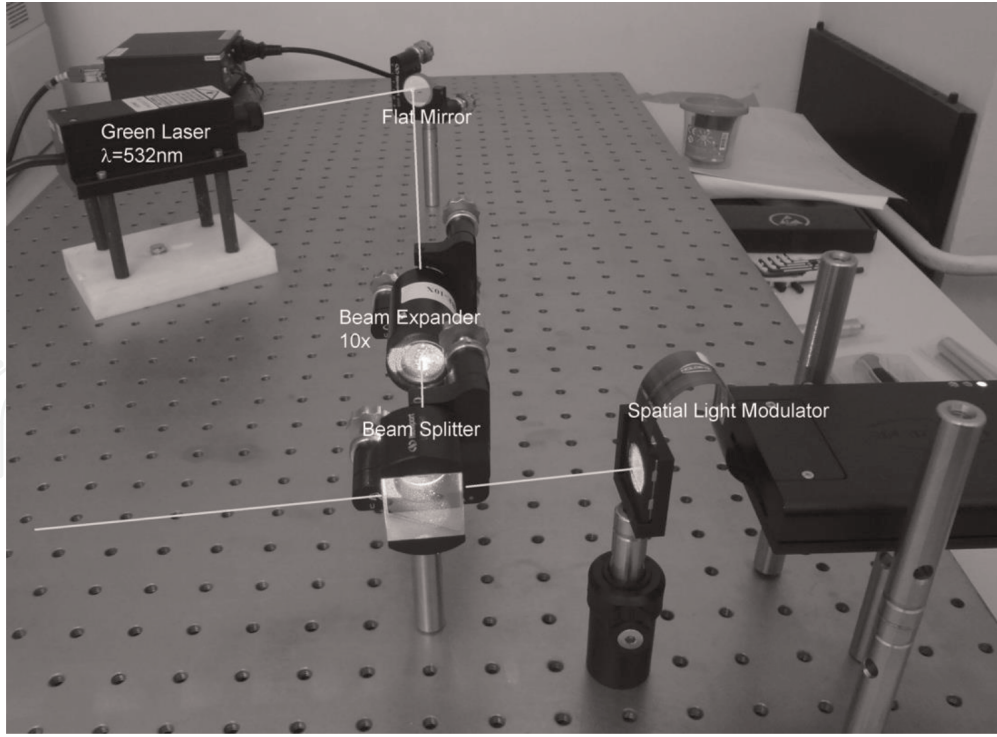
Figure 6. Assembled optical setup for optical experiments.
