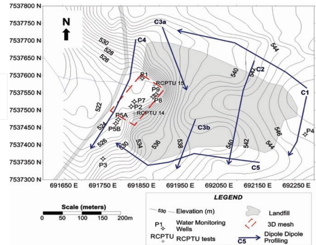
Figure 17. Topographical map of the landfill with the location of monitoring wells, soundings, and the 3D geophysical survey mesh.
