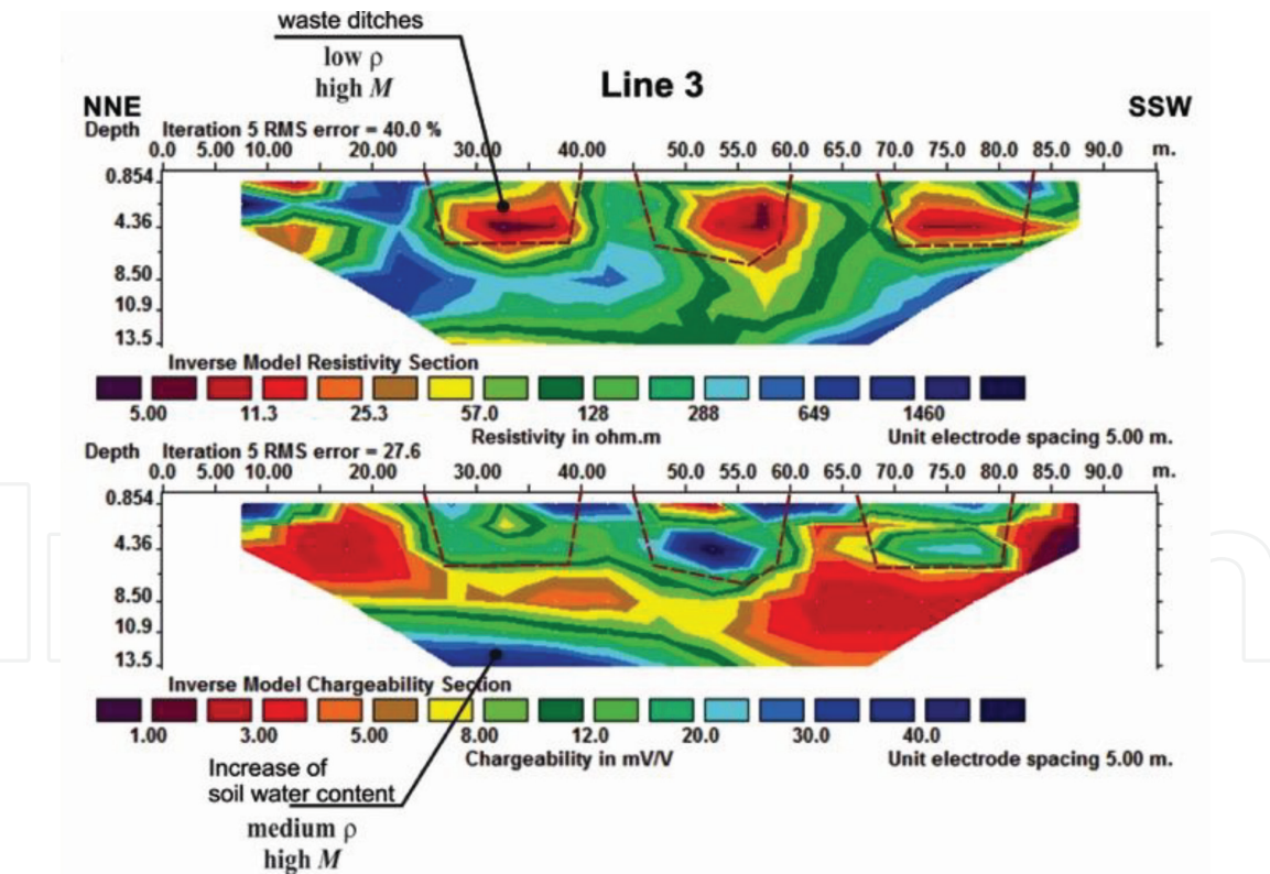
Figure 14. Resistivity and chargeability sessions perpendicular to the landfill ditches.
