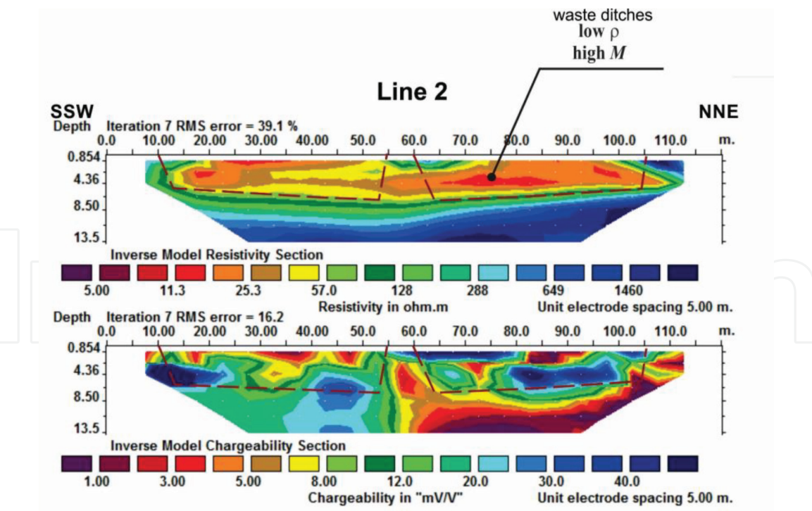
Figure 13. Resistivity and chargeability sessions of Line 2.
