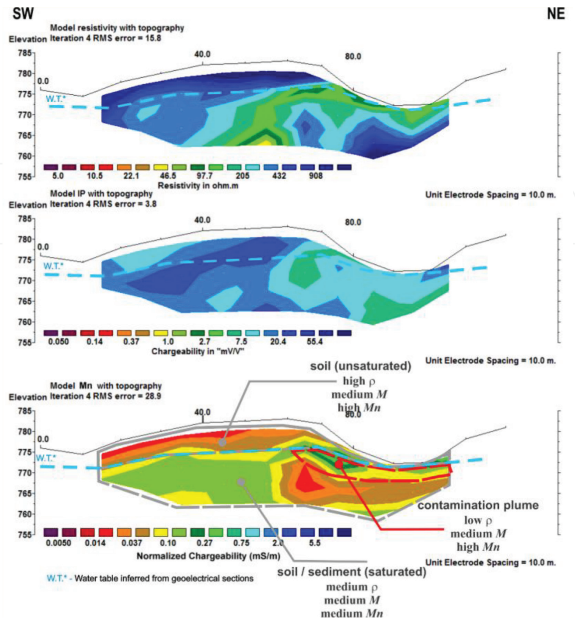
Figure 11. Resistivity (top), chargeability (middle), and normalized chargeability (bottom) sections of Line 0.
