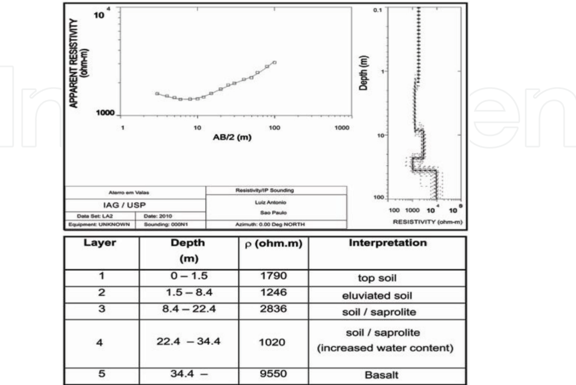
Figure 16. Interpretation of VES2.
