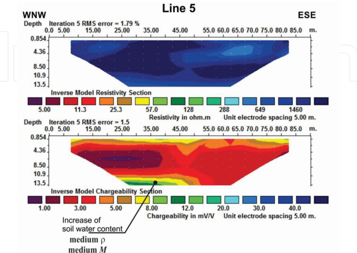
Figure 15. Resistivity and chargeability sessions south from the trench landfill.
