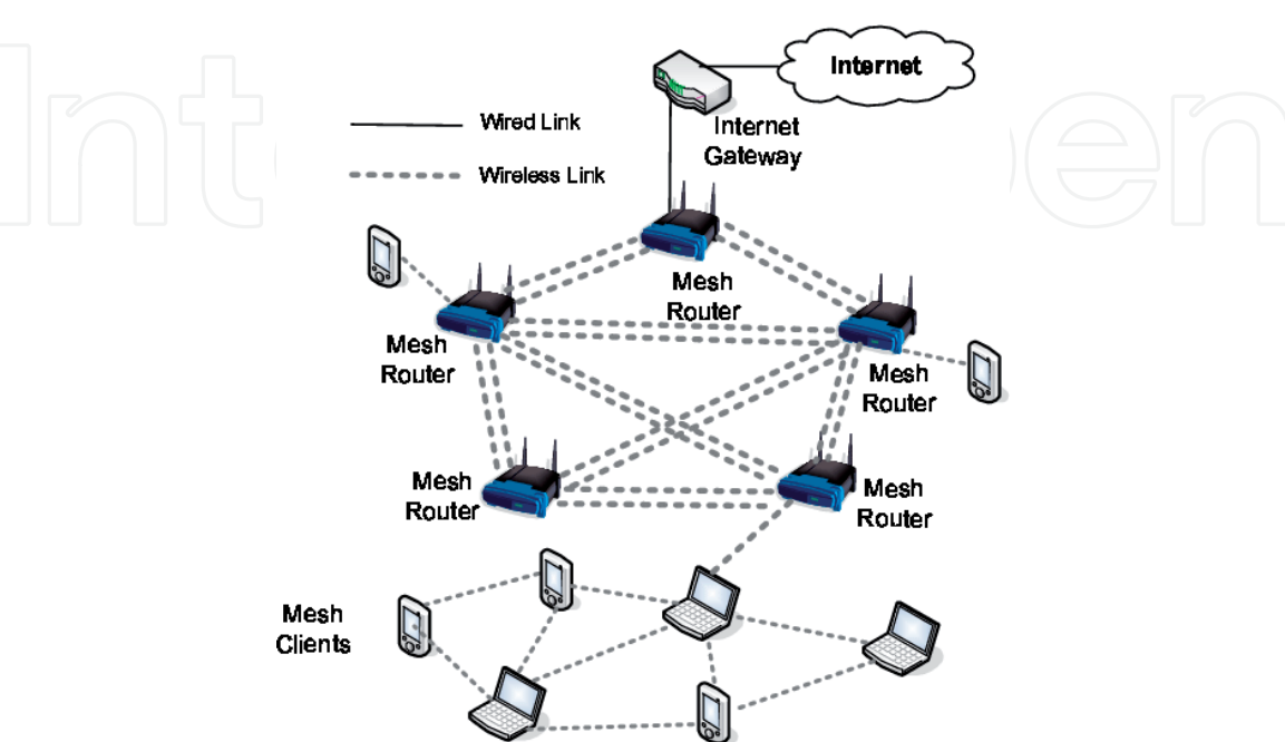
Figure 3. Hybrid mesh architecture.
