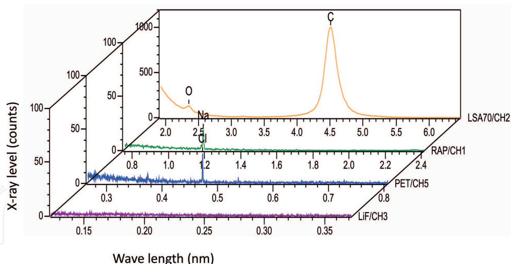
Figure 2. Result of qualitative analysis by EPMA.
