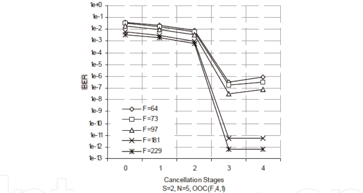
Figure 7. The BER of the Opt-SIC system versus the cancellation stage for different code lengths and for threshold value equal to 2.
