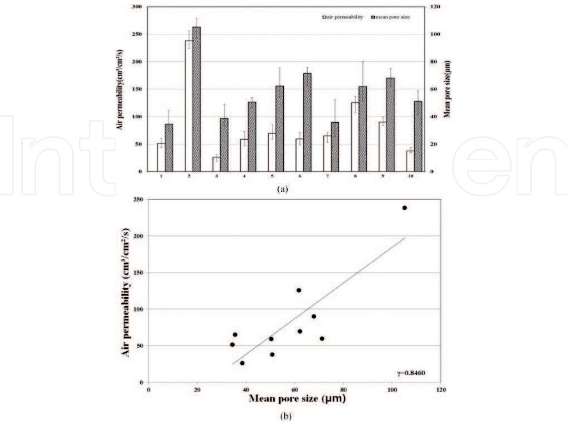
Figure 16. Air permeability of the nonwoven specimens. (a) Air permeability of each specimens and (b) Air permeability vs Mean pore size.
