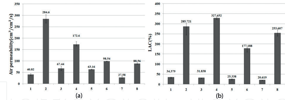
Figure 22. Air permeability and water absorption of the kenaf-imbedded nonwoven treated and non-treated with laminated PU film. (a) Air permeability and (b) Water absorption.
