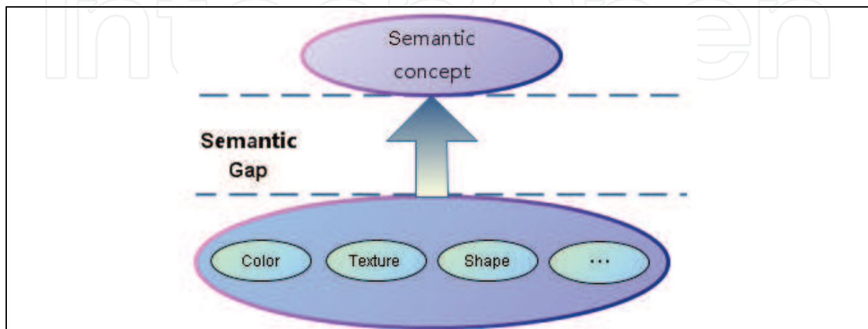
Fig. 8. Semantic Gap
