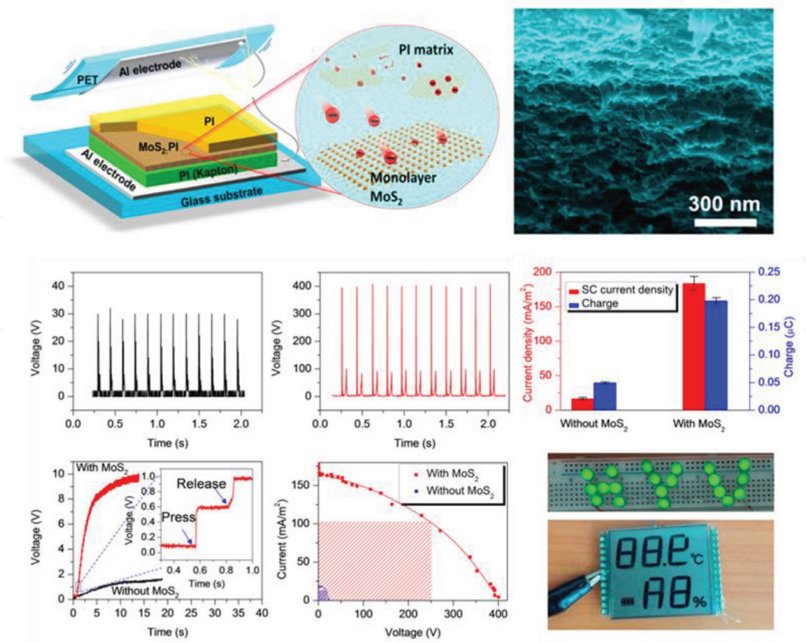
Figure 4. A contact-separation mode TENG with monolayer MoS 2 [21].
