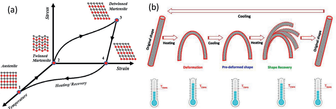
Figure 2. Schematic diagram of (a) stress-strain-temperature for the involved crystallographic changes during the phenomena of SME [5], (b) one-way SME for SMPs.
