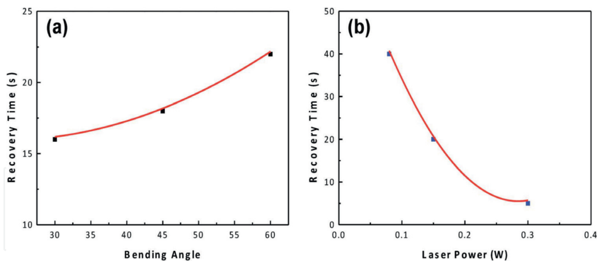
Figure 17. Recovery time versus (a) bending angle and (b) laser power, of the reinforced SMPs with AuNRs at 45° pillar angle [49].
