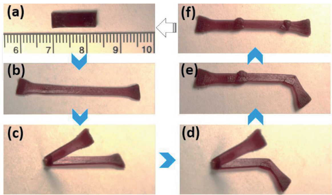
Figure 18. Optical observation of the shape transformation of cross-linked PEO film reinforced with AuNPs using a laser as a temperature source; (a) original film, (b) deformed sample at 80 °C, (c) large-out of plane bending, (d) gradient chain relaxation and (e,f) shape recovery after applying the laser heating source.
