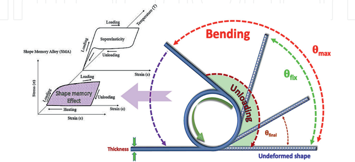
Figure 5. Schematic drawing of bending test as thermomechanical cycles test.
