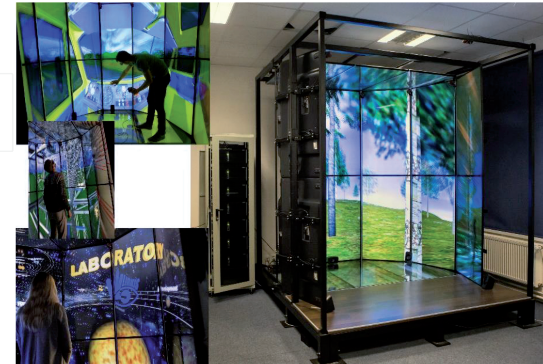
Figure 1. Virtual cave in laboratory LIRKIS at technical University of Košice and the examples of immersive visualization in this environment.
