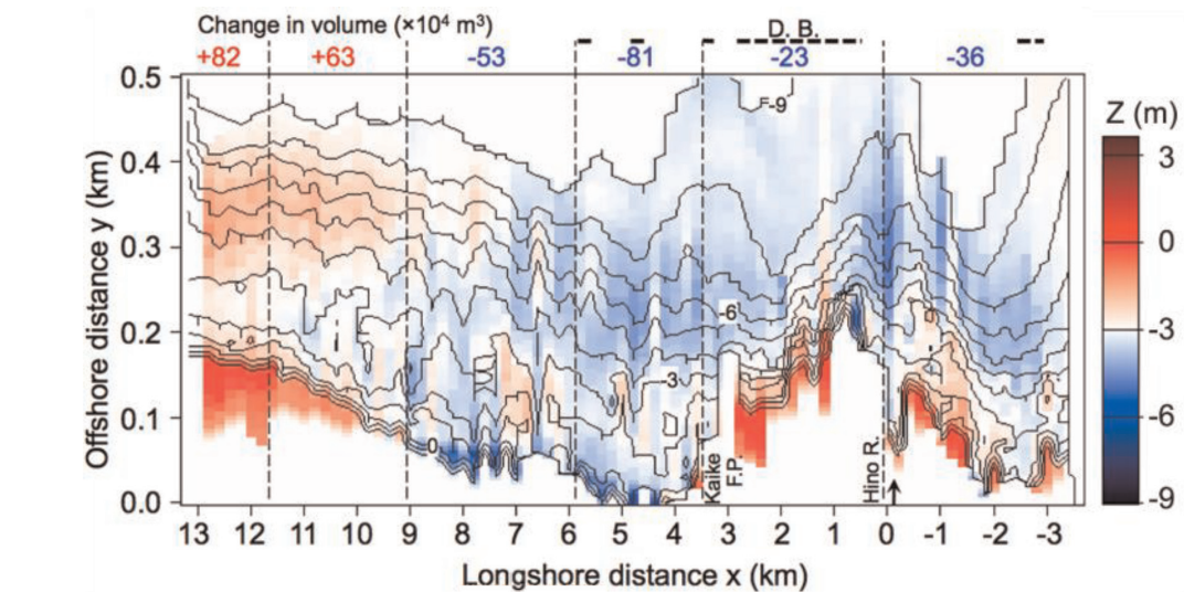
Figure 5. Bathymetry in 2000 using expanded coordinates and bathymetric changes with reference to that in 1980.
