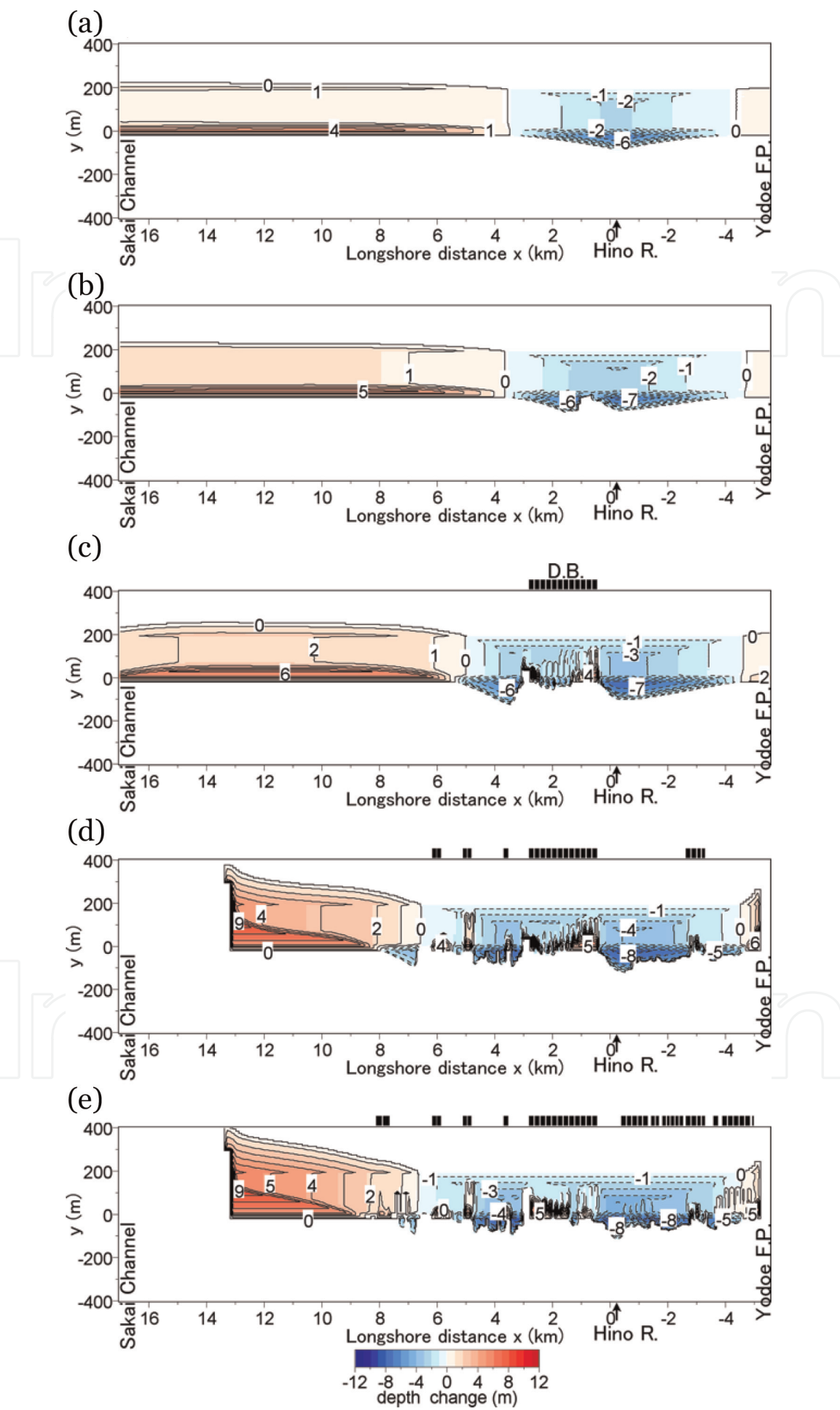
Figure A2. Bathymetric changes with reference to bathymetry in 1947. (a) 1962. (b) 1967. (c) 1980. (d) 1995. (e) 2010.
