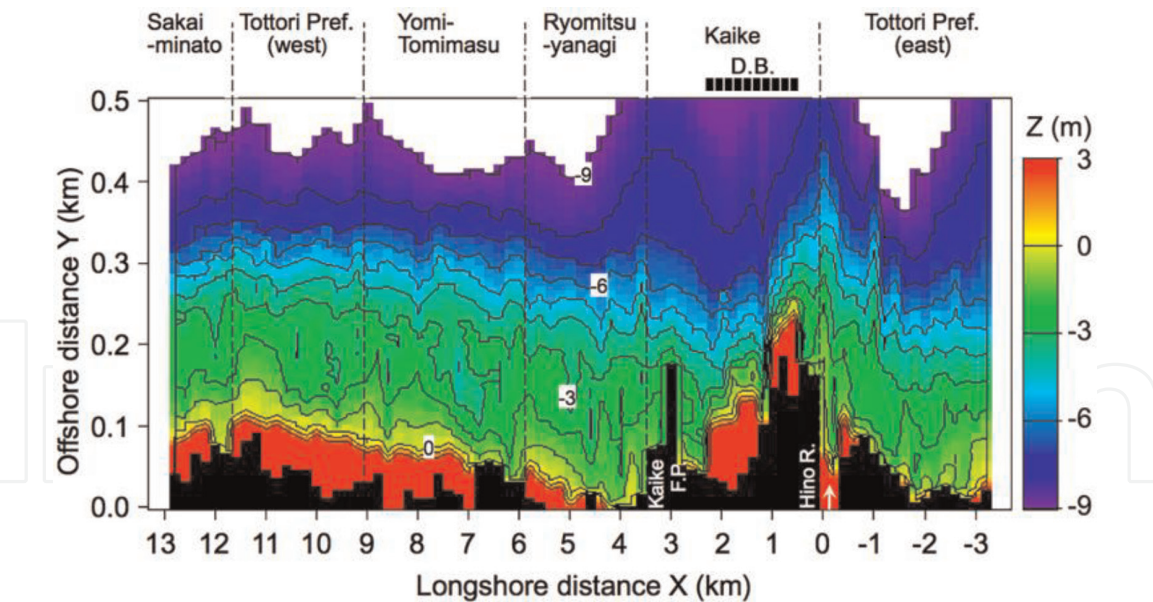
Figure 4. Bathymetry in 1980 using expanded coordinates.
