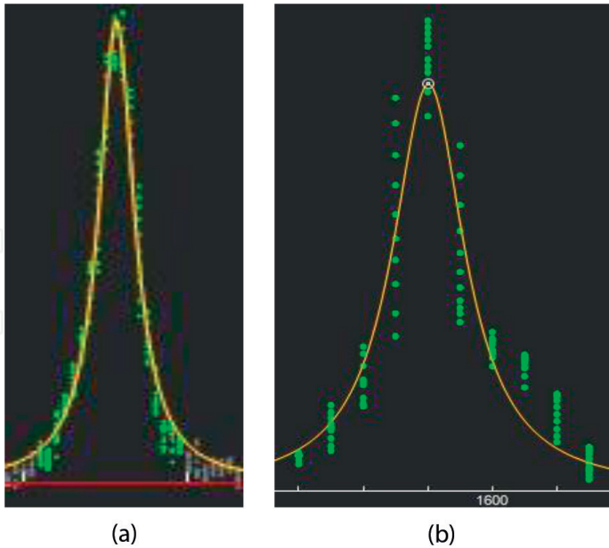
Figure 11. (a) D-band on left (Intensity: 33.5, Center: 1312.4 cm -1 ), (b) G-band on right (Intensity: 62.5, Center: 1580.2 cm -1 ) for graphene nanoplatelets (ammonia) with 780 nm excitation and using fityk peak fitting software [14].
