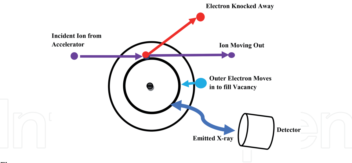
Figure 4. Schematic of PIXE setup.
