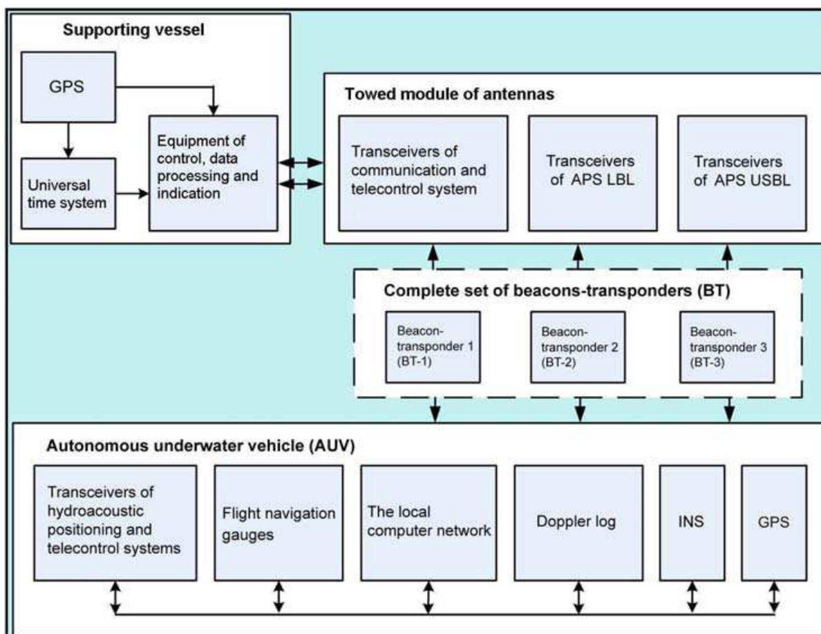
Fig. 1. AUV positioning devices
