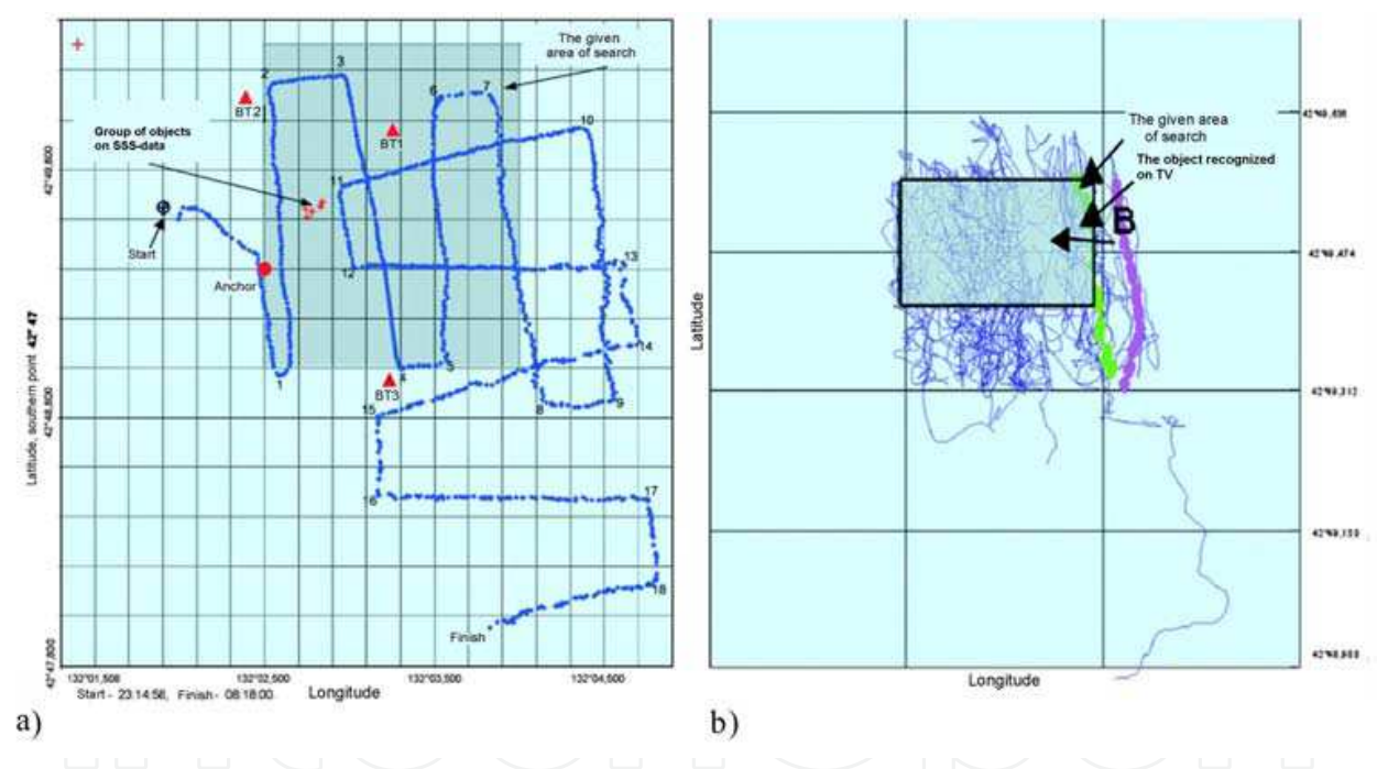
Fig. 2. Area path investigation during helicopter search. a) large-scale SSS survey, S = 22 \text{ sq. km} , \Delta = 20 \text{ m} ; b) detailed video survey, S = 0.16 \text{ sq. km} , \Delta = 5 \text{ m}
