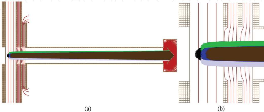
Figure 5. (a) Trajectory simulated for naphthalene ( \text{C}_{10}\text{H}_8 ) with 480\text{ }\mu\text{m}/\mu\text{s} velocity from different position (colored as blue, green, black, white, brown) in the interaction region (b) Particle distribution in the interaction region. Red contours are the equipotential lines.
