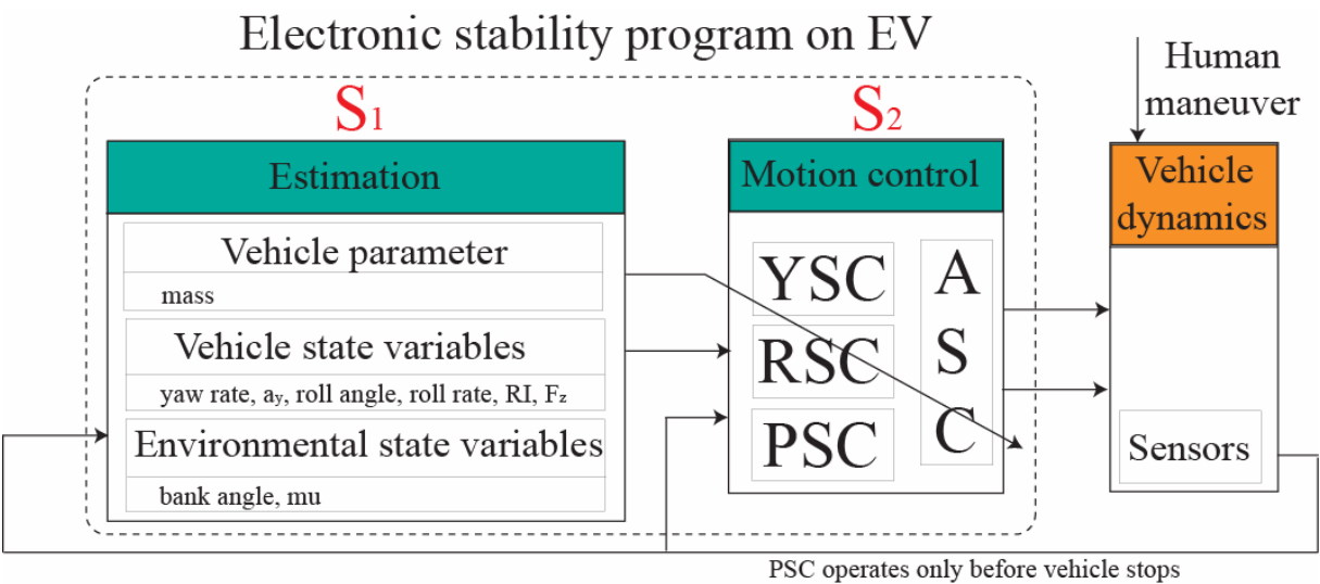
Fig. 1. EPS based on DOB
