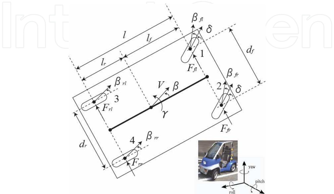
Fig. 3. Four wheel model
