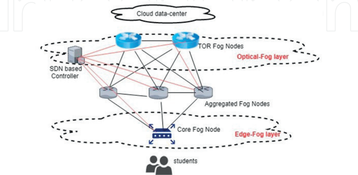
Figure 6. SDN-based Optical-Fog network.
