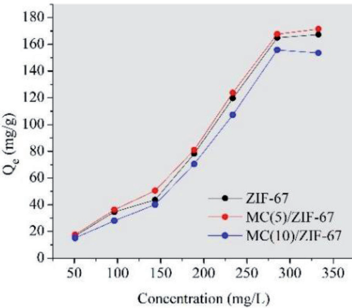
Figure 8. Effect of initial concentrations of MO.
