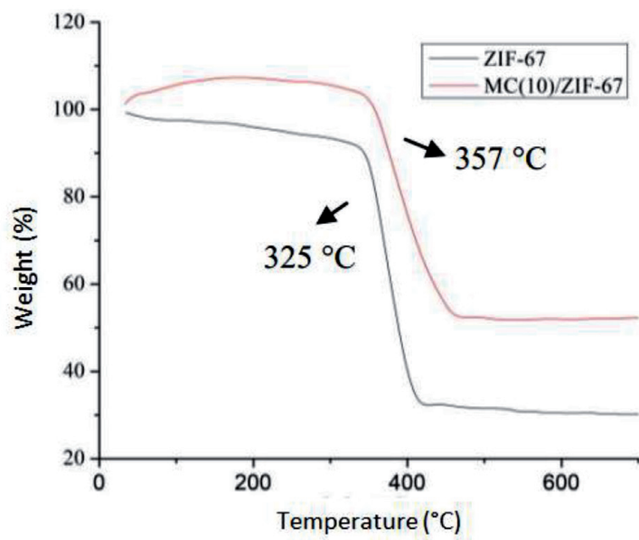
Figure 5. Thermogravimetric profiles of ZIF-7 and MC(10)/ZIF-67 composite.
