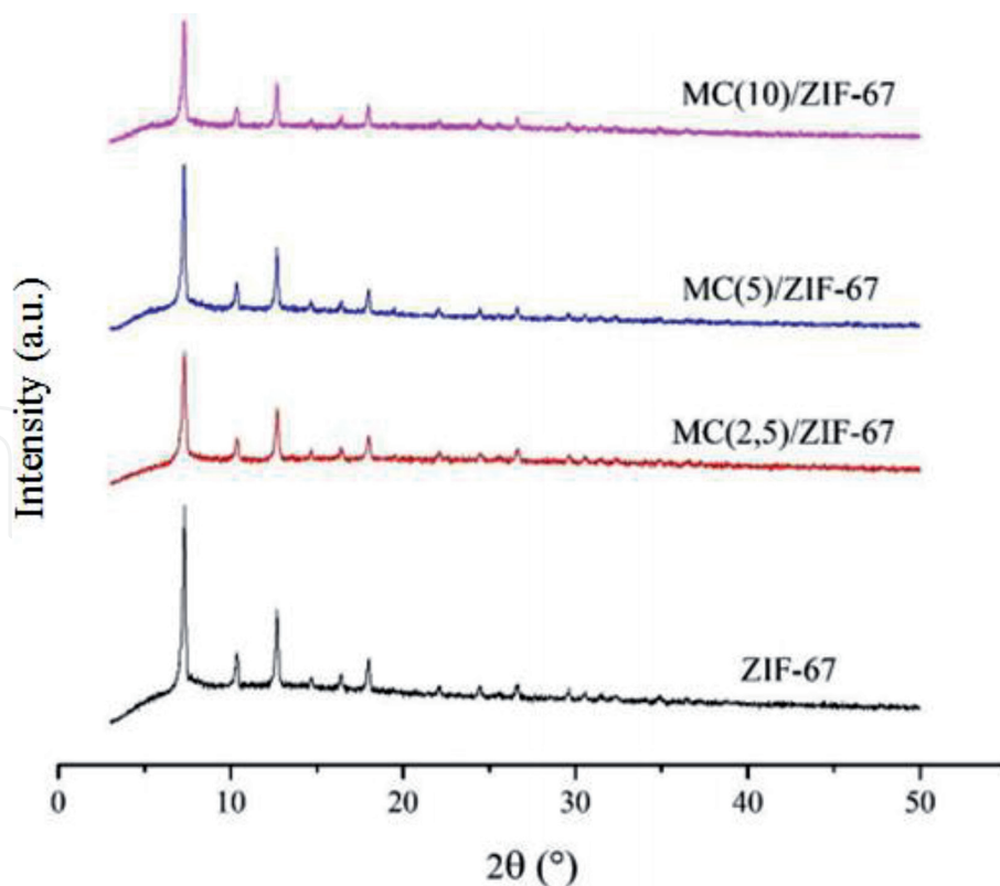
Figure 1. XRD pattern of ZIF-67 and MCM-41/ZIF-67 composites.
