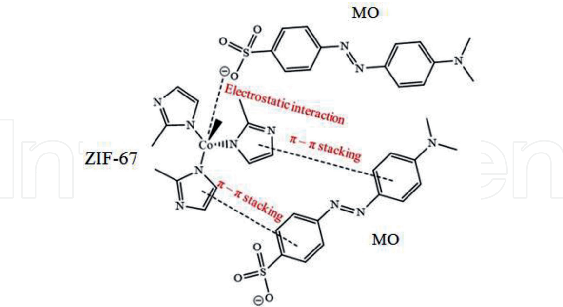
Figure 10. Mechanism of MO adsorption to ZIF-67.
