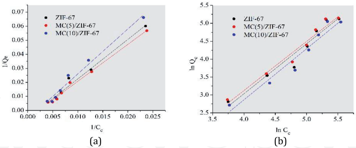
Figure 9. Plots of (a) Langmuir and (b) Freundlich models of MO adsorption.
