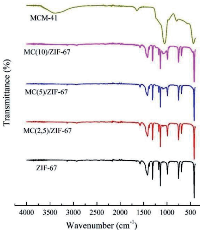
Figure 2. FT-IR spectra of ZIF-67 and the composites.
