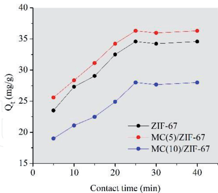
Figure 6. Effect of contact time on MO adsorption.
